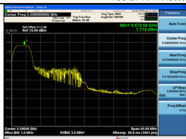
Mode:802.11ax HE40 Tone:52T Frequency:5590MHz Ant:Chain0
