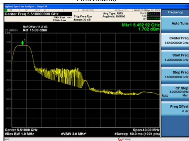
Mode:802.11ax HE40 Tone:52T Frequency:5510MHz Ant:Chain1
