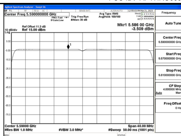
Mode:802.11ax HE40 Tone:484T Frequency:5590MHz Ant:Chain0
