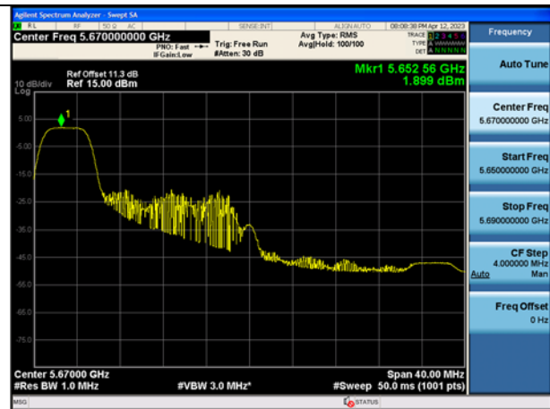
Mode:802.11ax HE40 Tone:52T Frequency:5670MHz Ant:Chain1
