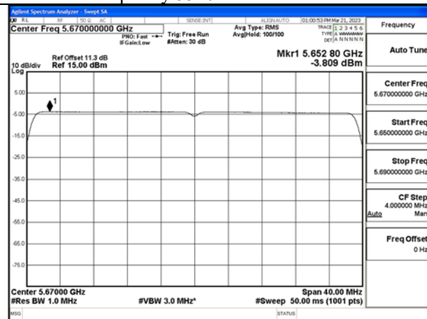
Mode:802.11ax HE40 Tone:484T Frequency:5670MHz Ant:Chain1
