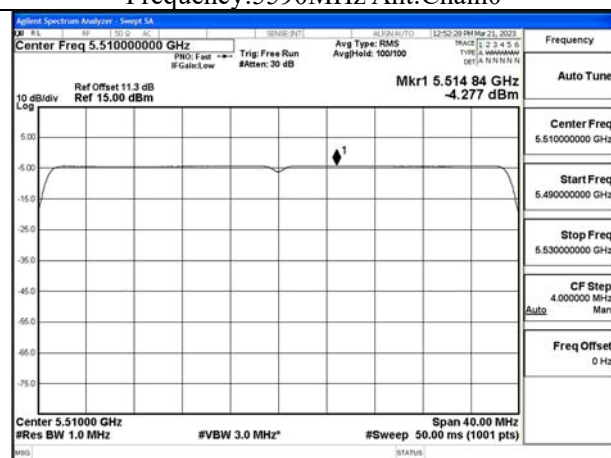
Mode:802.11ax HE40 Tone:484T Frequency:5510MHz Ant:Chain1
