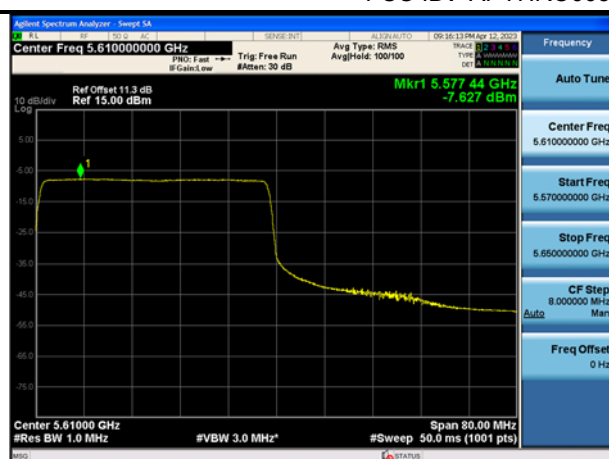
Mode:802.11ax HE80 Tone:484T Frequency:5610MHz Ant:Chain1
