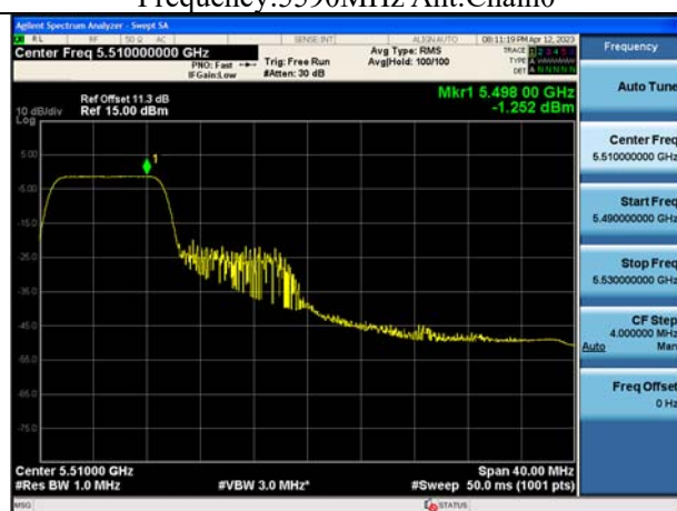
Mode:802.11ax HE40 Tone:106T Frequency:5510MHz Ant:Chain1
