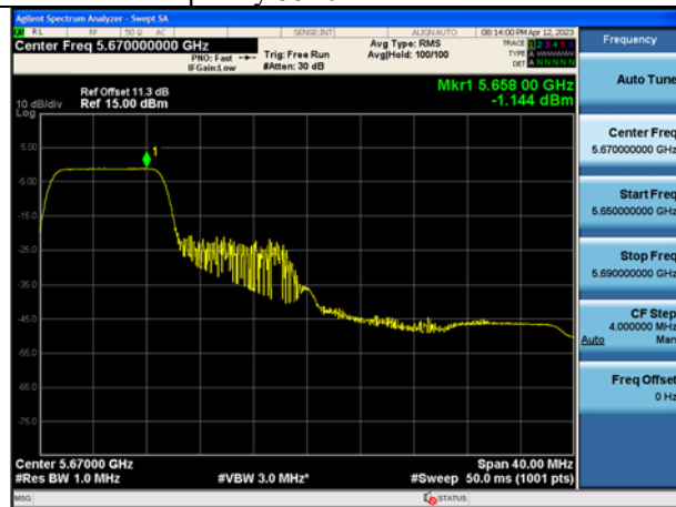
Mode:802.11ax HE40 Tone:106T Frequency:5670MHz Ant:Chain1
