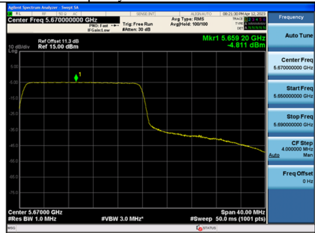
Mode:802.11ax HE40 Tone:242T Frequency:5670MHz Ant:Chain1
