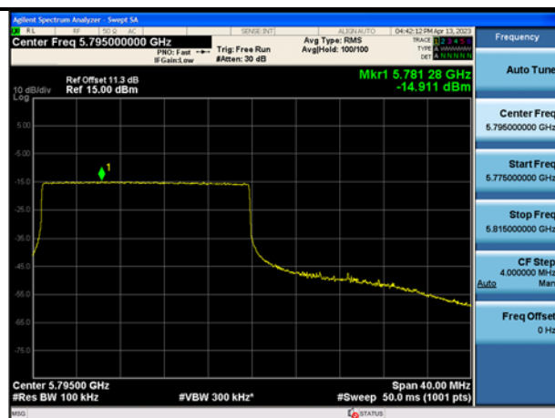
Mode:802.11ax HE40 Tone:242T Frequency:5795MHz Ant:Chain0
