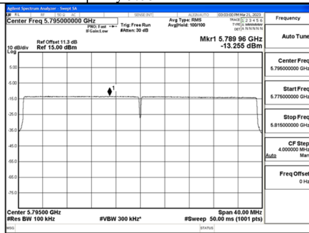
Mode:802.11ax HE40 Tone:484T Frequency:5795MHz Ant:Chain0
