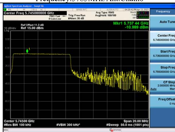
Mode:802.11ax HE20 Tone:106T Frequency:5745MHz Ant:Chain1
