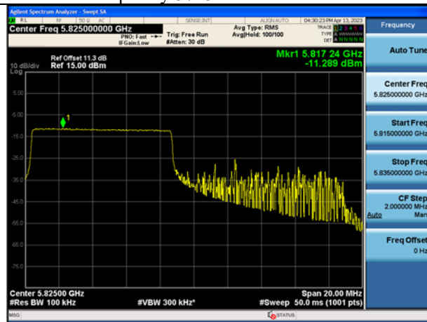
Mode:802.11ax HE20 Tone:106T Frequency:5825MHz Ant:Chain1
