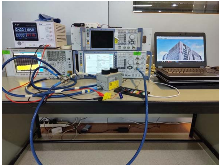
RF Conducted Test setup (GSM/WCDMA)
