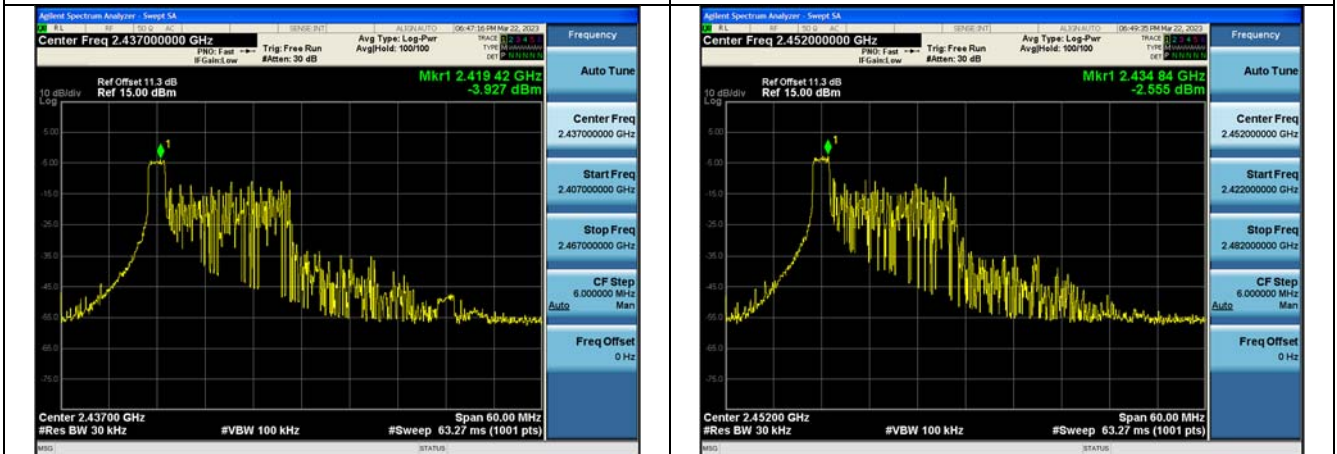
Test Mode:802.11ax HE40 2437MHz Chain1
