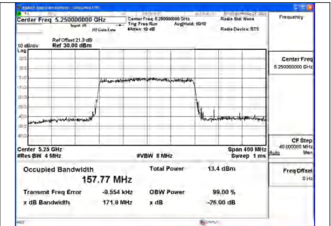
Test Mode:802.11ax HE160 5250MHz Chain1
