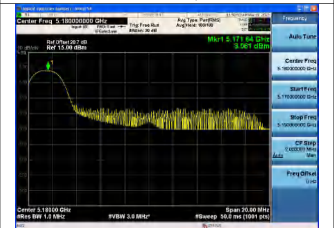
Mode:802.11ax HE20 Tone:26T Frequency:5180MHz Ant:Chain1
