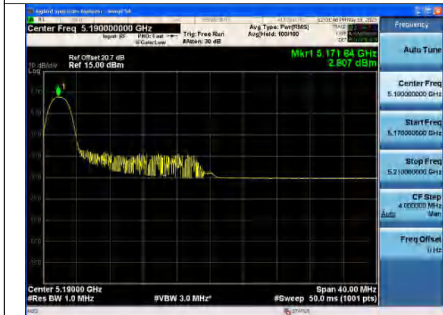
Mode:802.11ax HE40 Tone:26T Frequency:5190MHz Ant:Chain1
