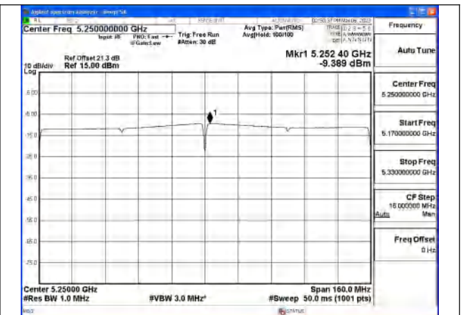
Mode:802.11ax HE160 Tone:1992T Frequency:5250MHz Ant:Chain1
