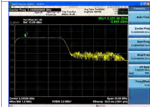
Mode:802.11ax HE20 Tone:106T Frequency:5240MHz Ant:Chain0
