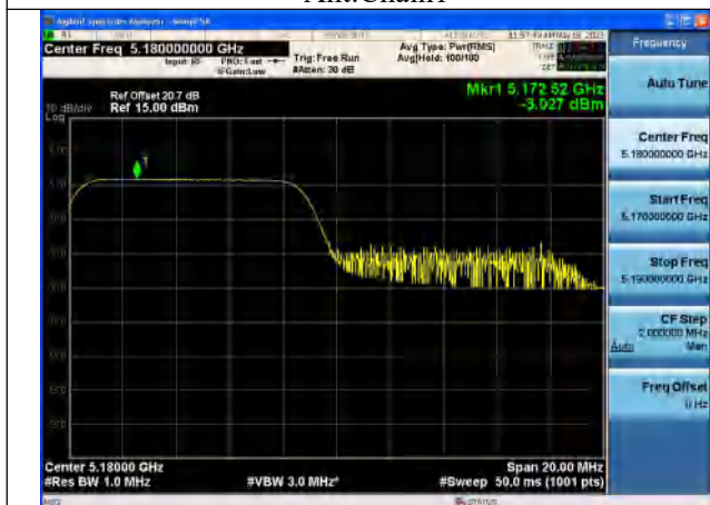
Mode:802.11ax HE20 Tone:106T Frequency:5180MHz Ant:Chain0
