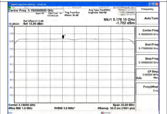
Mode:802.11ax HE20 Tone:242T Frequency:5180MHz Ant:Chain1
