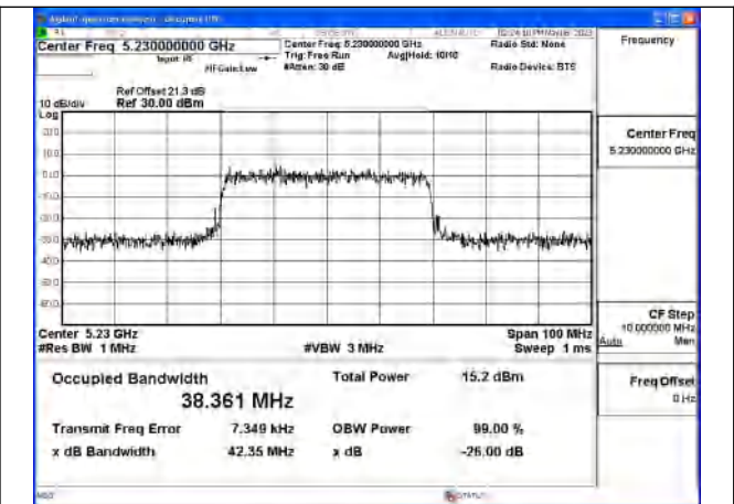
Test Mode:802.11ax HE40 5230MHz Chain0
