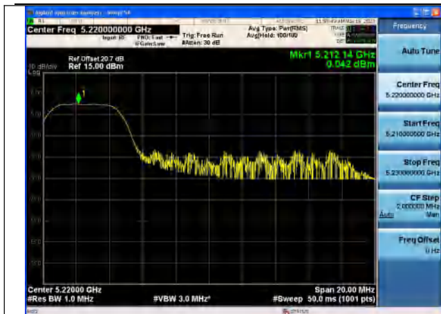
Mode:802.11ax HE20 Tone:52T Frequency:5220MHz Ant:Chain1
