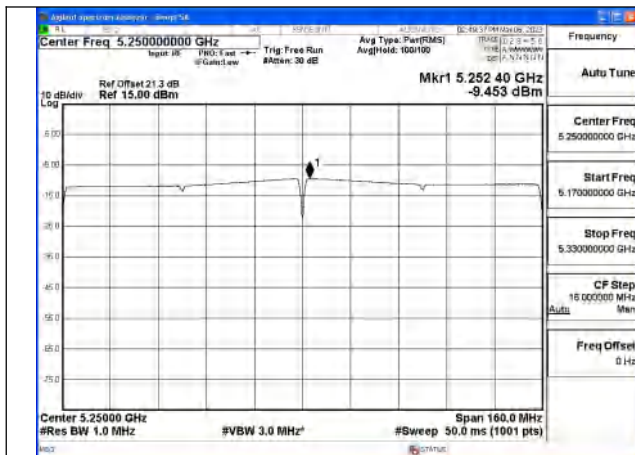
Mode:802.11ax HE160 Tone:1992T Frequency:5250MHz Ant:Chain0
