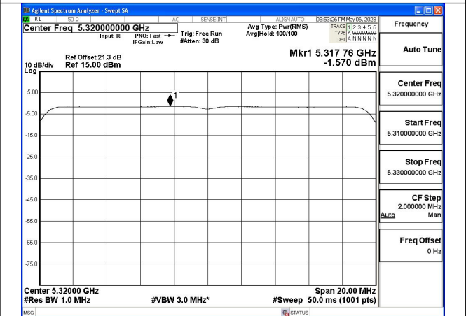
Mode:802.11ax HE20 Tone:242T Frequency:5320MHz Ant:Chain1
