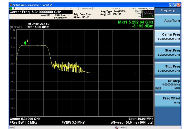
Mode:802.11ax HE40 Tone:106T Frequency:5310MHz Ant:Chain1
