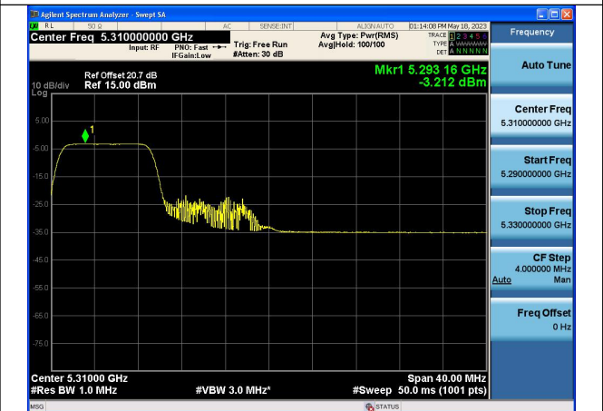
Mode:802.11ax HE40 Tone:106T Frequency:5310MHz Ant:Chain0
