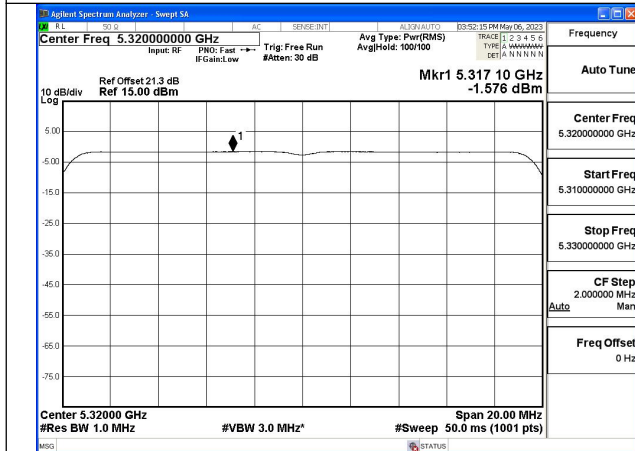
Mode:802.11ax HE20 Tone:242T Frequency:5320MHz Ant:Chain0
