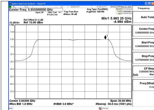
Mode:802.11ax HE20 Tone:242T Frequency:5955MHz Chain0
