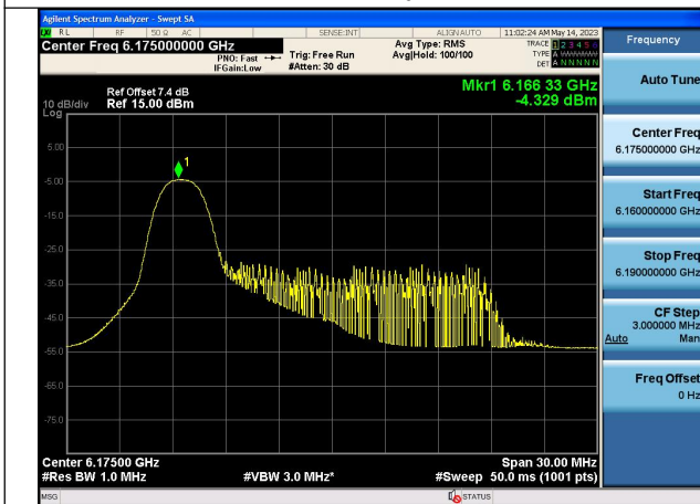
Mode:802.11ax HE20 Tone:26T Frequency:6175MHz Chain1
