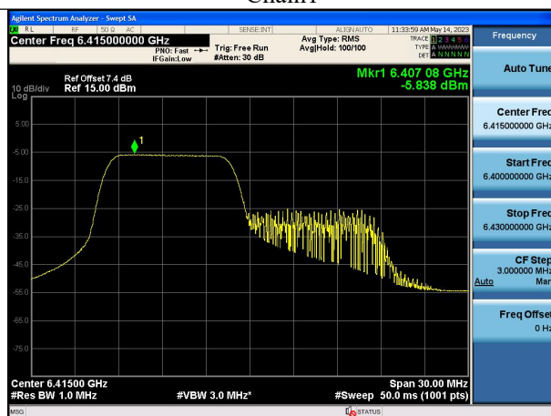
Mode:802.11ax HE20 Tone:106T Frequency:6415MHz Chain1
