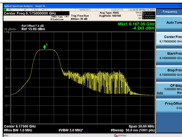
Mode:802.11ax HE20 Tone:52T Frequency:6175MHz Chain0
