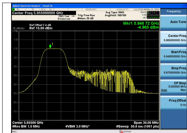
Mode:802.11ax HE20 Tone:52T Frequency:5955MHz Chain0
