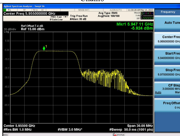
Mode:802.11ax HE20 Tone:106T Frequency:5955MHz Chain1
