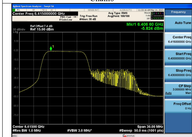
Mode:802.11ax HE20 Tone:106T Frequency:6415MHz Chain0
