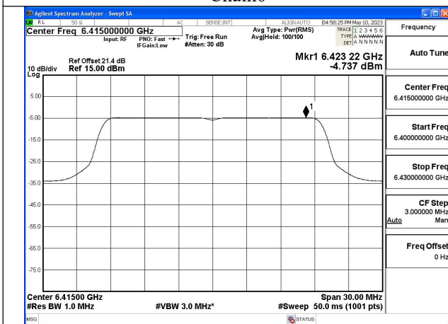
Mode:802.11ax HE20 Tone:242T Frequency:6415MHz Chain0
