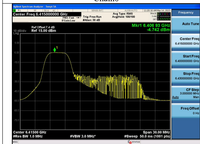
Mode:802.11ax HE20 Tone:52T Frequency:6415MHz Chain0
