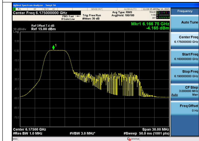
Mode:802.11ax HE20 Tone:52T Frequency:6175MHz Chain1
