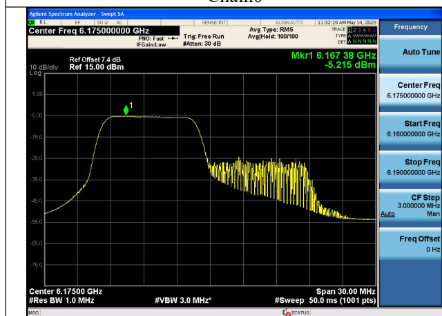
Mode:802.11ax HE20 Tone:106T Frequency:6175MHz Chain1
