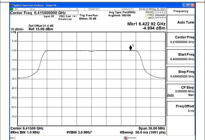
Mode:802.11ax HE20 Tone:242T Frequency:6415MHz Chain1
