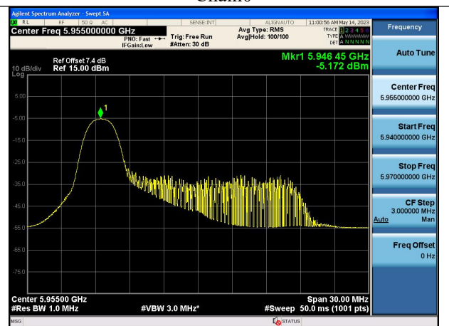
Mode:802.11ax HE20 Tone:26T Frequency:5955MHz Chain1
