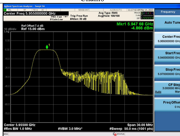
Mode:802.11ax HE20 Tone:52T Frequency:5955MHz Chain1
