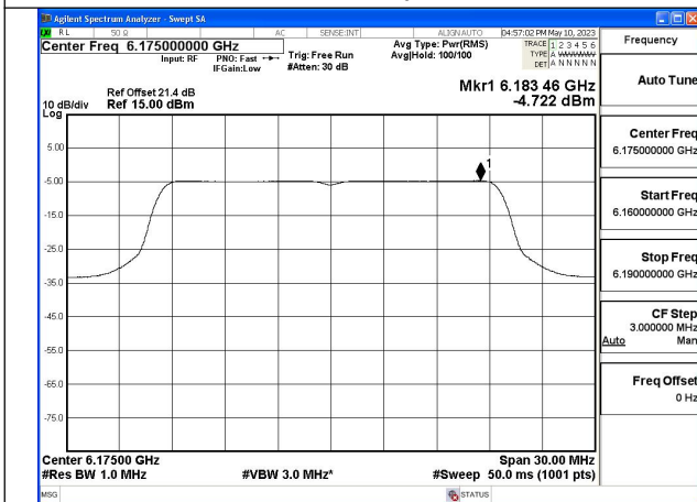
Mode:802.11ax HE20 Tone:242T Frequency:6175MHz Chain1
