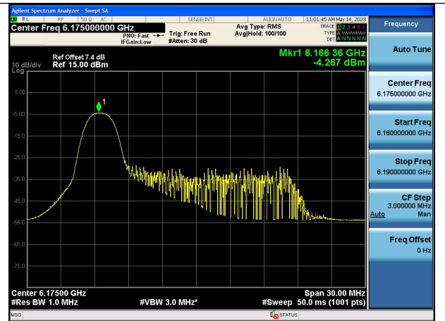
Mode:802.11ax HE20 Tone:26T Frequency:6175MHz Chain0
