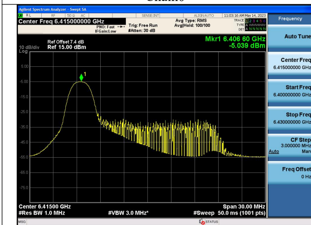
Mode:802.11ax HE20 Tone:26T Frequency:6415MHz Chain0
