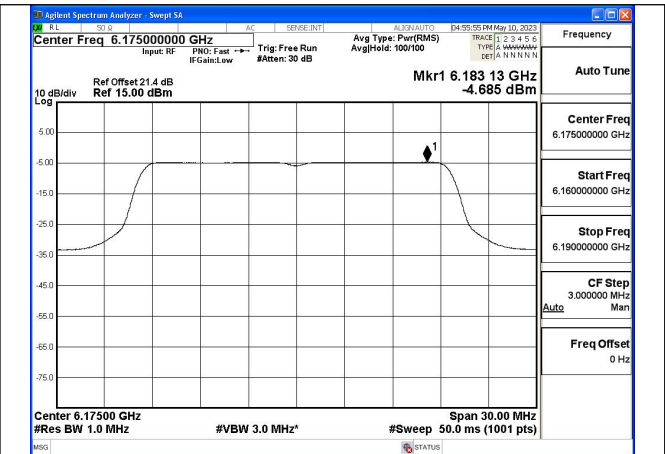
Mode:802.11ax HE20 Tone:242T Frequency:6175MHz Chain0
