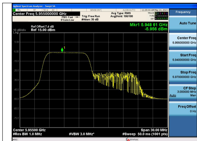
Mode:802.11ax HE20 Tone:106T Frequency:5955MHz Chain0
