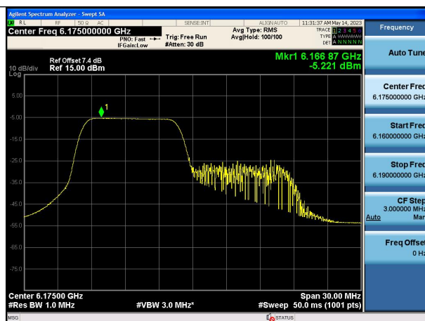
Mode:802.11ax HE20 Tone:106T Frequency:6175MHz Chain0
