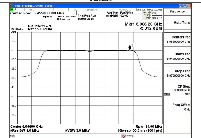
Mode:802.11ax HE20 Tone:242T Frequency:5955MHz Chain1
