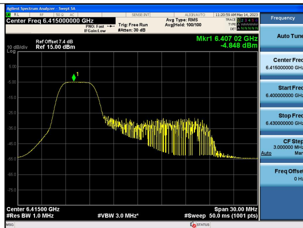
Mode:802.11ax HE20 Tone:52T Frequency:6415MHz Chain1
