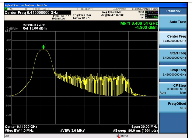
Mode:802.11ax HE20 Tone:26T Frequency:6415MHz Chain1
