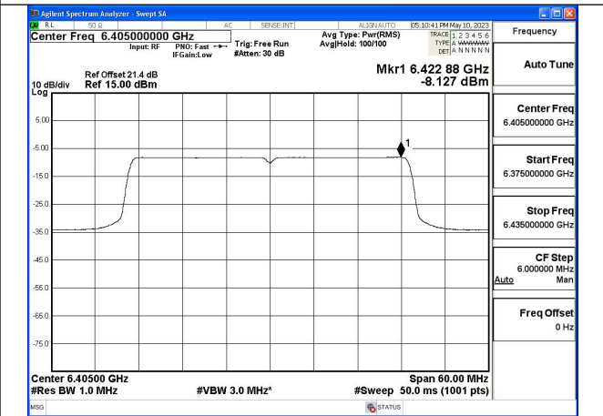
Mode:802.11ax HE40 Tone:484T Frequency:6405MHz Chain1
