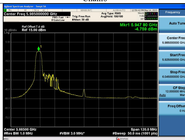
Mode:802.11ax HE80 Tone:52T Frequency:5985MHz Chain1
