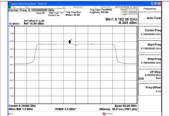
Mode:802.11ax HE40 Tone:484T Frequency:6165MHz Chain0
