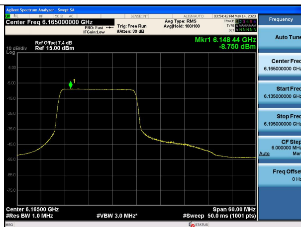
Mode:802.11ax HE40 Tone:242T Frequency:6165MHz Chain0
