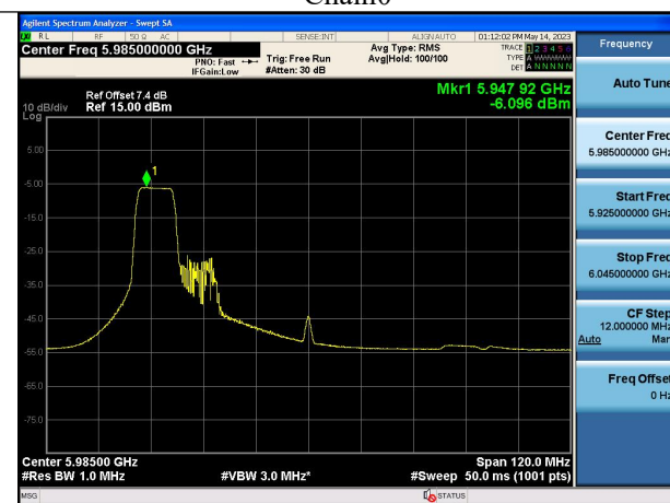
Mode:802.11ax HE80 Tone:106T Frequency:5985MHz Chain1
