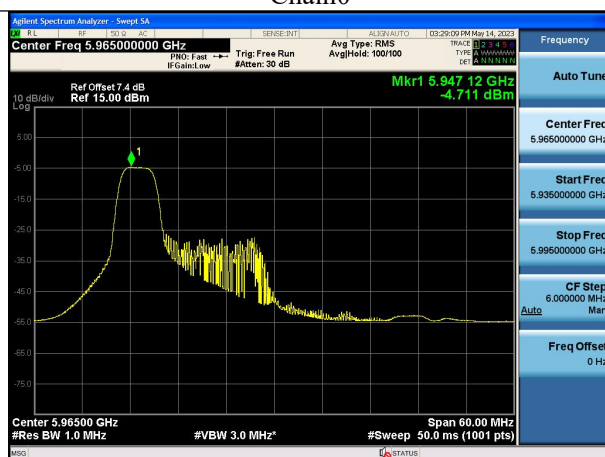
Mode:802.11ax HE40 Tone:52T Frequency:5965MHz Chain1
