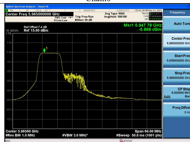
Mode:802.11ax HE40 Tone:106T Frequency:5965MHz Chain1
