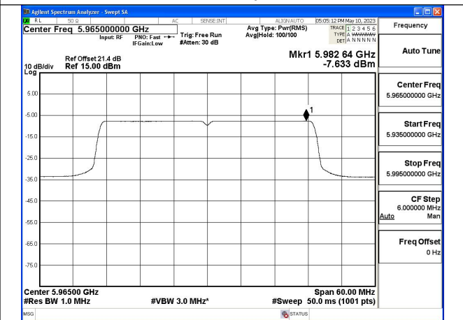
Mode:802.11ax HE40 Tone:484T Frequency:5965MHz Chain1
