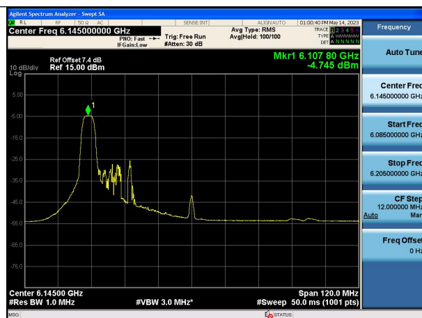
Mode:802.11ax HE80 Tone:52T Frequency:6145MHz Chain0
