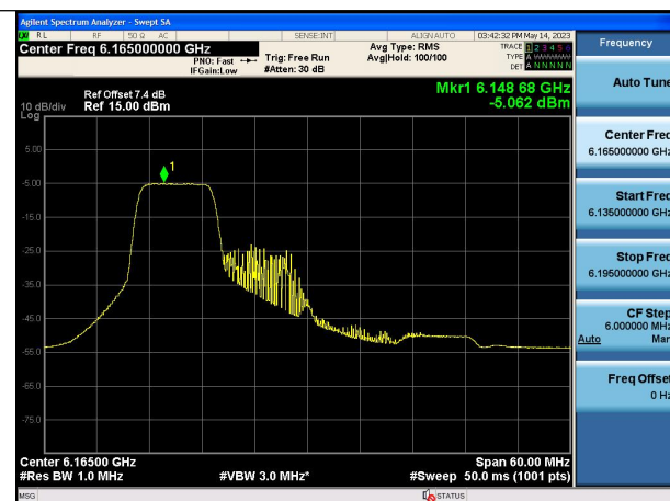
Mode:802.11ax HE40 Tone:106T Frequency:6165MHz Chain0
