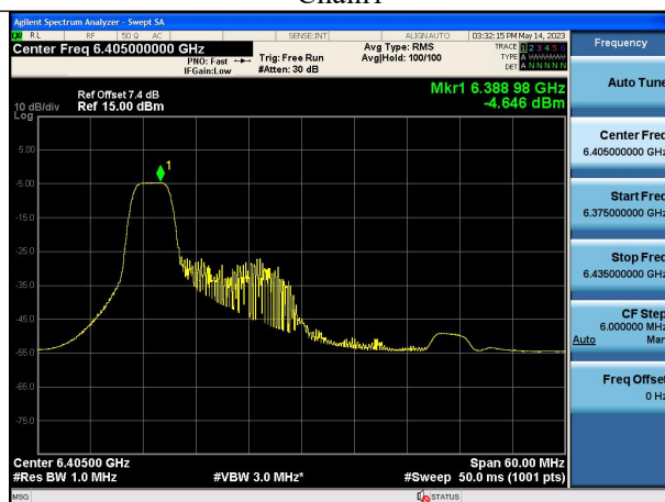
Mode:802.11ax HE40 Tone:52T Frequency:6405MHz Chain1
