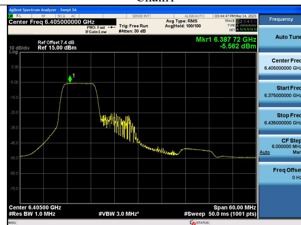
Mode:802.11ax HE40 Tone:106T Frequency:6405MHz Chain1
