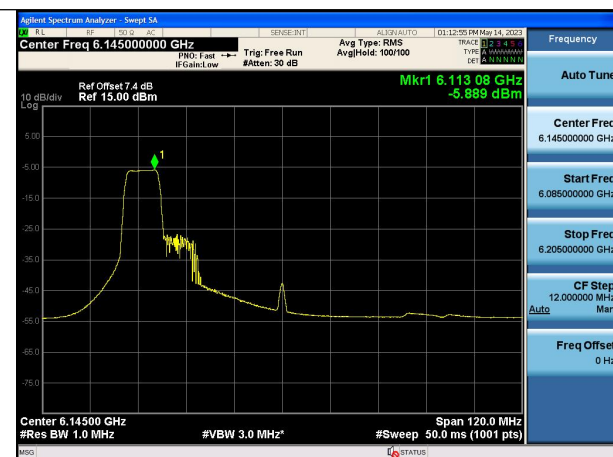
Mode:802.11ax HE80 Tone:106T Frequency:6145MHz Chain0
