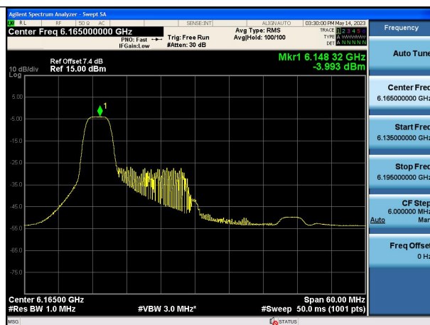
Mode:802.11ax HE40 Tone:52T Frequency:6165MHz Chain0
