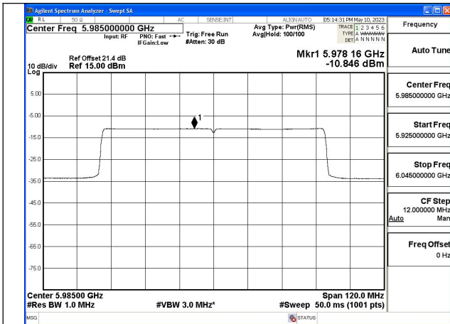
Mode:802.11ax HE80 Tone:996T Frequency:5985MHz Chain0
