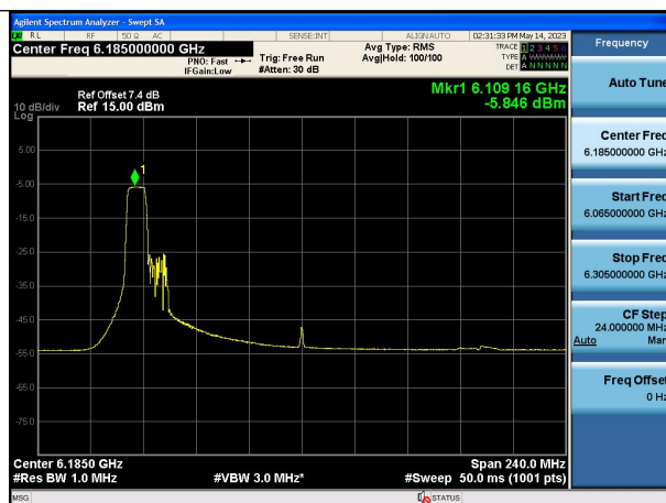
Mode:802.11ax HE160 Tone:106T Frequency:6185MHz Chain0
