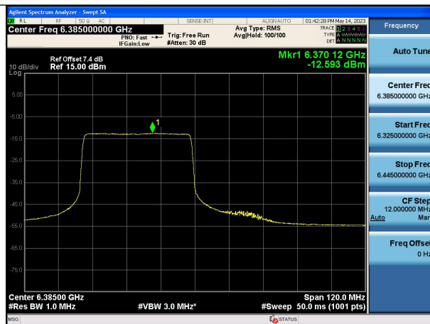
Mode:802.11ax HE80 Tone:484T Frequency:6385MHz Chain1
