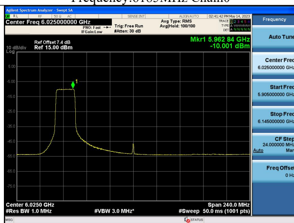
Mode:802.11ax HE160 Tone:242T Frequency:6025MHz Chain1
