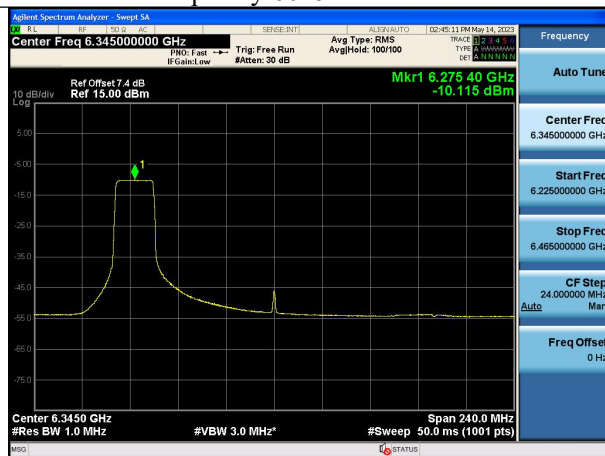
Mode:802.11ax HE160 Tone:242T Frequency:6345MHz Chain1
