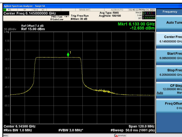
Mode:802.11ax HE80 Tone:484T Frequency:6145MHz Chain0
