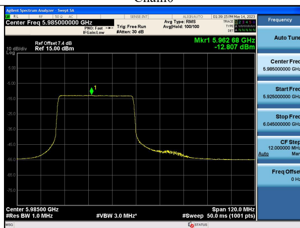
Mode:802.11ax HE80 Tone:484T Frequency:5985MHz Chain1
