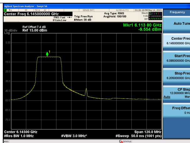
Mode:802.11ax HE80 Tone:242T Frequency:6145MHz Chain0
