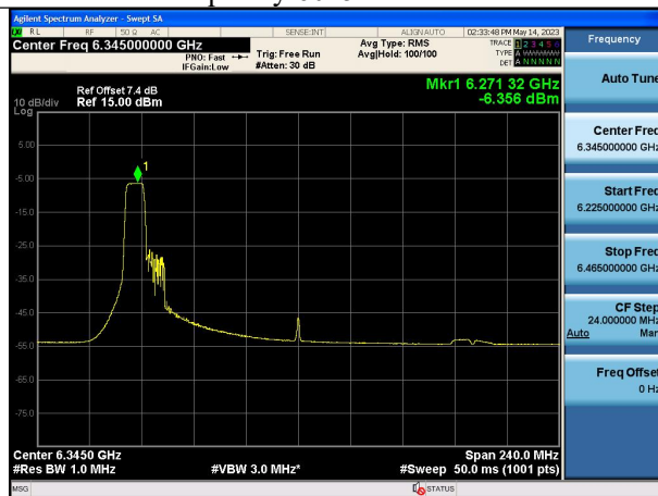
Mode:802.11ax HE160 Tone:106T Frequency:6345MHz Chain1
