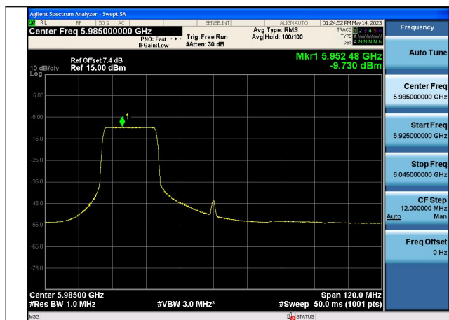
Mode:802.11ax HE80 Tone:242T Frequency:5985MHz Chain0
