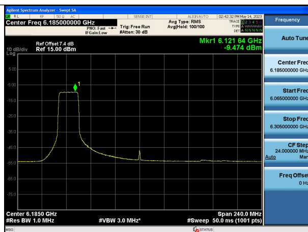
Mode:802.11ax HE160 Tone:242T Frequency:6185MHz Chain0
