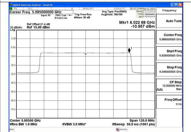
Mode:802.11ax HE80 Tone:996T Frequency:5985MHz Chain1
