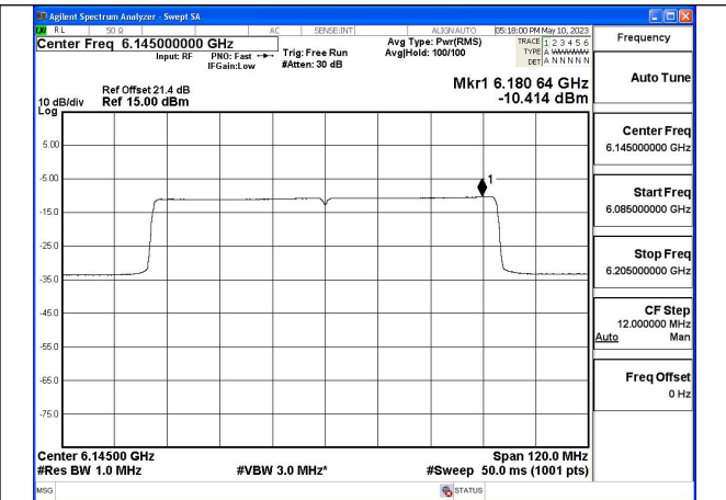
Mode:802.11ax HE80 Tone:996T Frequency:6145MHz Chain0
