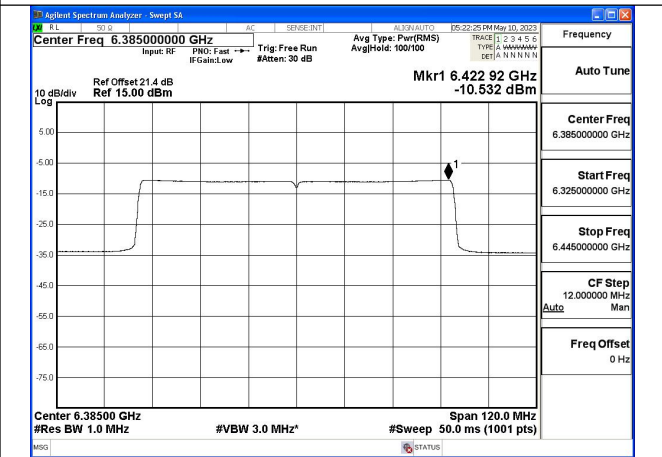
Mode:802.11ax HE80 Tone:996T Frequency:6385MHz Chain1
