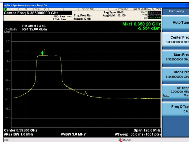
Mode:802.11ax HE80 Tone:242T Frequency:6385MHz Chain1
