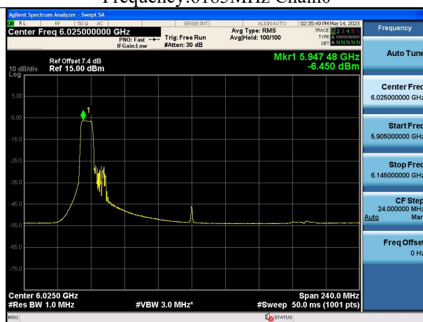
Mode:802.11ax HE160 Tone:106T Frequency:6025MHz Chain1
