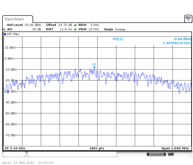
Power Density (dBm/3kHz) Plot Channel 19
