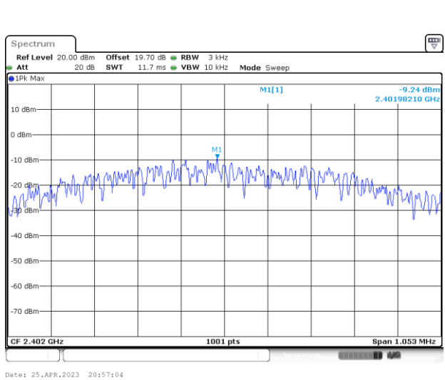
Power Density (dBm/3kHz) Plot Channel 00
