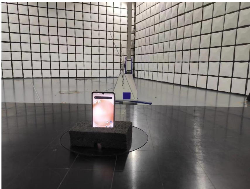
RE 30MHz~1GHz
