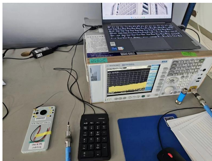
RF Conducted Test setup (BT/WIFI)
