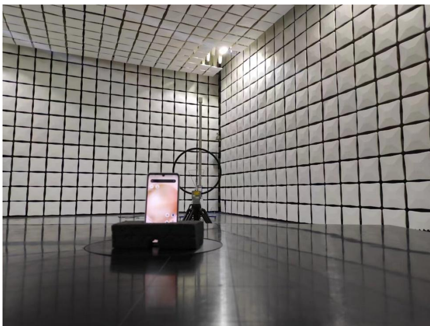
RE 9KHz~30MHz
