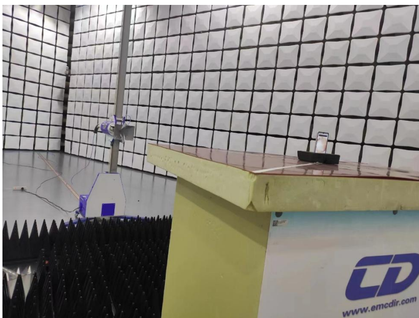
RE >1GHz
