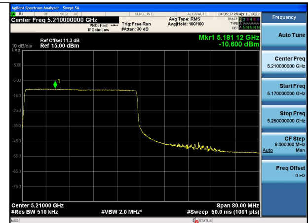
Mode:802.11ax HE80 Tone:484T Frequency:5210MHz Ant:Chain1
