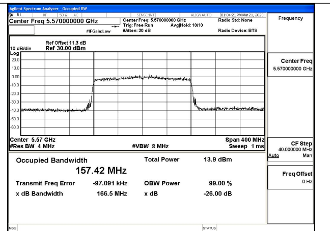
Test Mode:802.11ax HE160 5570MHz Chain1
