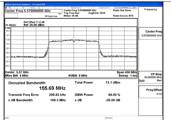
Test Mode:802.11ac VHT160 5570MHz Chain1
