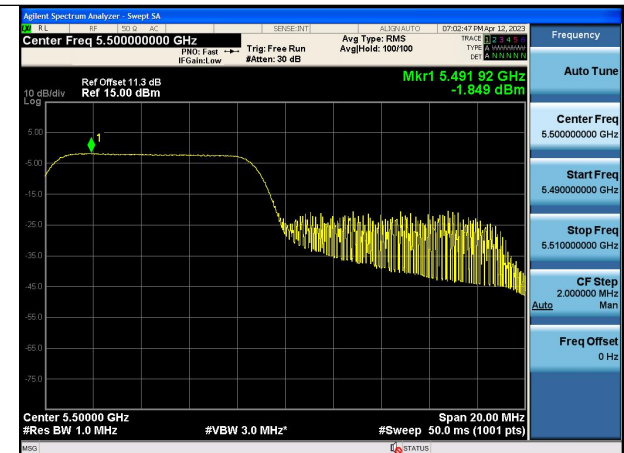
Mode:802.11ax HE20 Tone:106T Frequency:5500MHz Ant:Chain1
