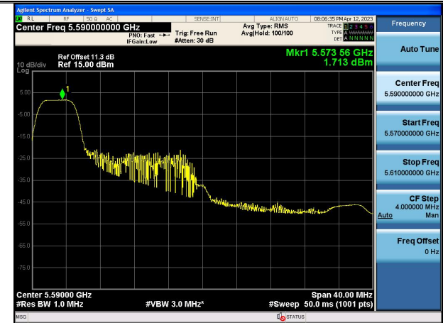
Mode:802.11ax HE40 Tone:52T Frequency:5590MHz Ant:Chain0
