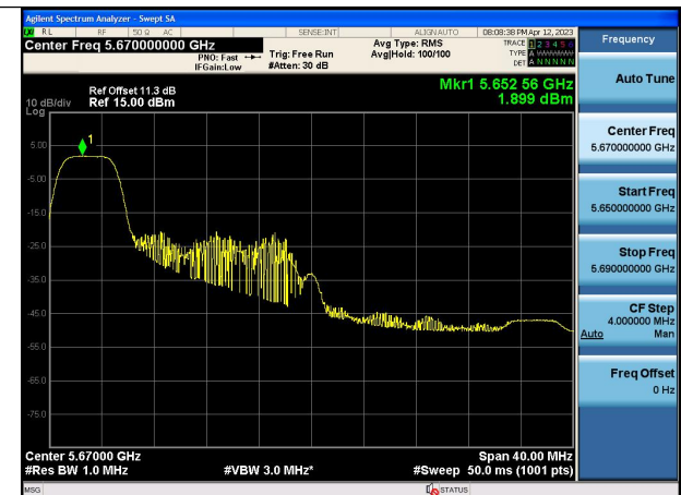
Mode:802.11ax HE40 Tone:52T Frequency:5670MHz Ant:Chain1
