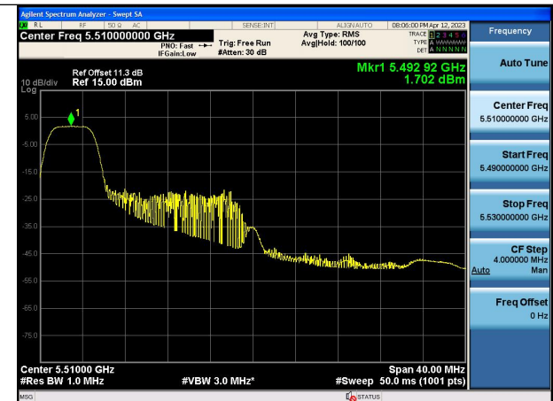
Mode:802.11ax HE40 Tone:52T Frequency:5510MHz Ant:Chain1
