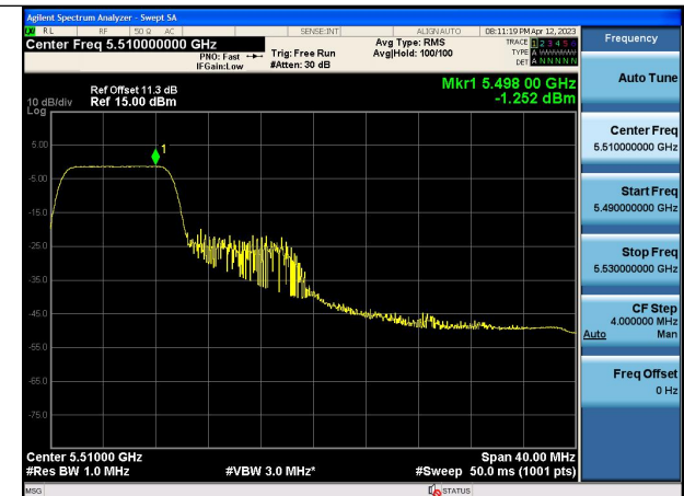
Mode:802.11ax HE40 Tone:106T Frequency:5510MHz Ant:Chain1
