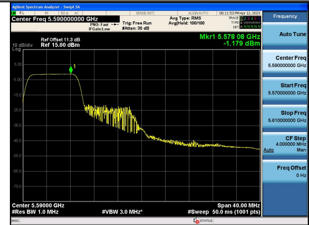
Mode:802.11ax HE40 Tone:106T Frequency:5590MHz Ant:Chain0
