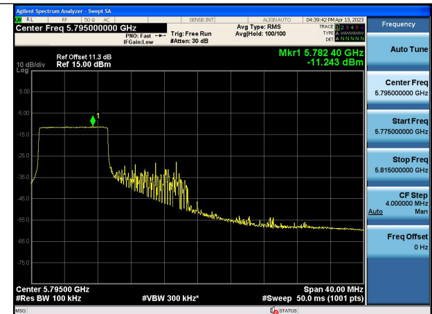
Mode:802.11ax HE40 Tone:106T Frequency:5795MHz Ant:Chain0
