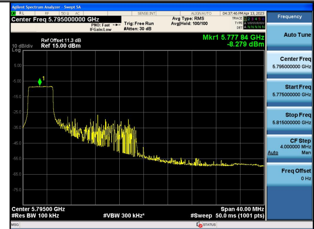
Mode:802.11ax HE40 Tone:52T Frequency:5795MHz Ant:Chain1
