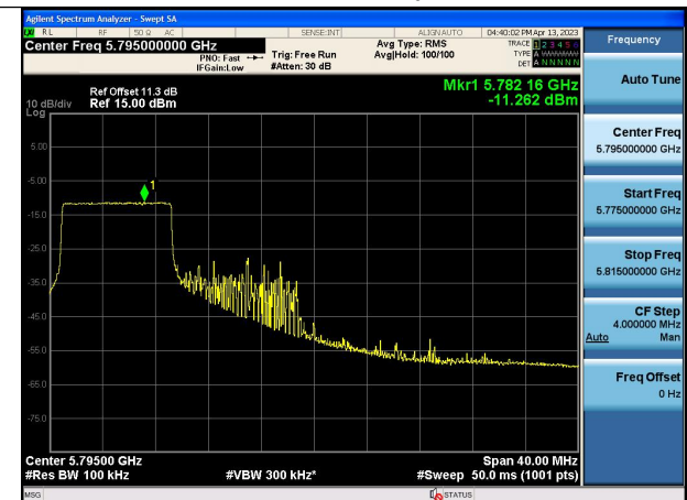
Mode:802.11ax HE40 Tone:106T Frequency:5795MHz Ant:Chain1
