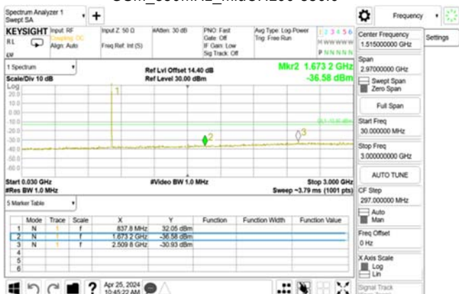
GSM_850MHz_MidCH190-836.6
