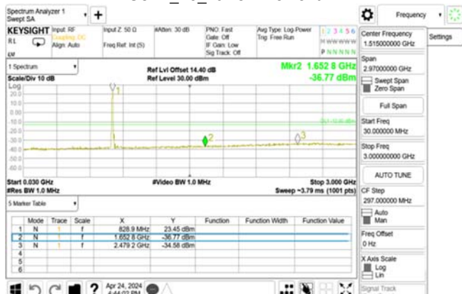
HSUPA_B5_LowCH4132-826.4
