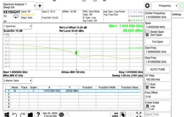
Band Edge HSDPA_B2_HighCH9538-1907.6
