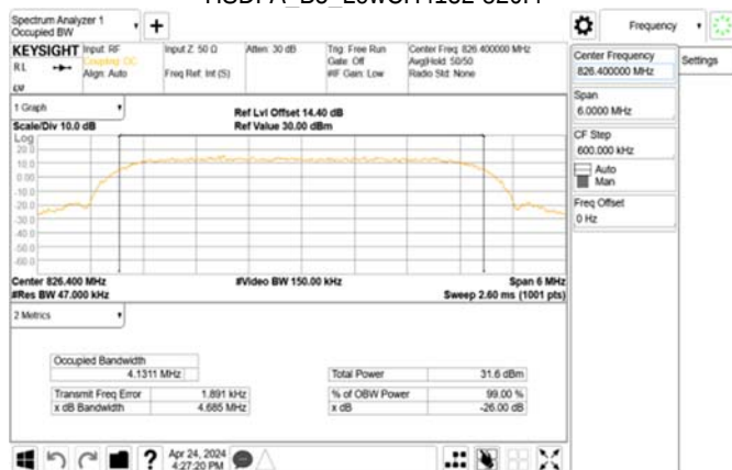
HSDPA_B5_LowCH4132-826.4
