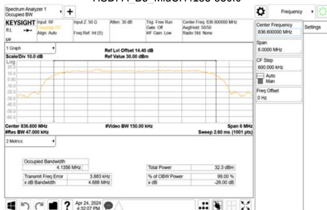
HSDPA_B5_MidCH4183-836.6
