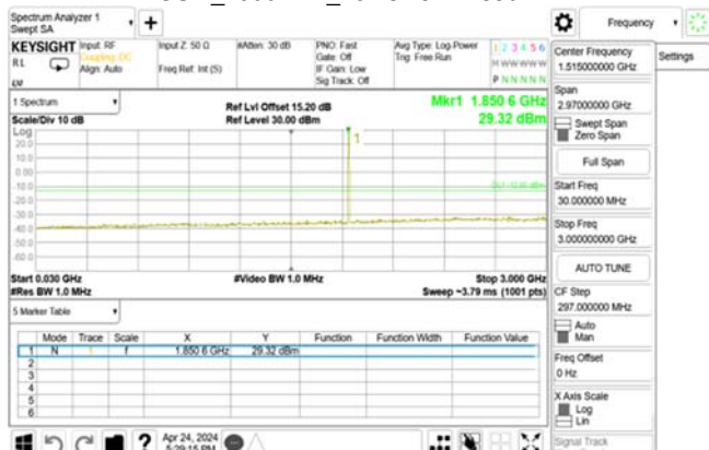
GSM_1900MHz_LowCH512-1850.2
