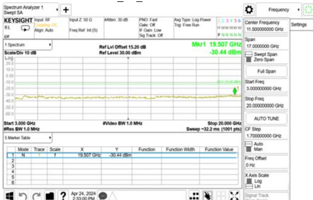
HSDPA_B2_MidCH9400-1880
