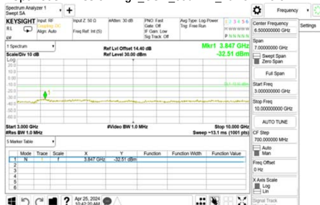
Spurious Emission High_GSM_850MHz_LowCH128-824.2
