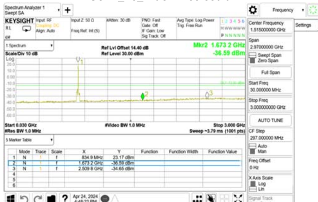
HSUPA_B5_MidCH4183-836.6
