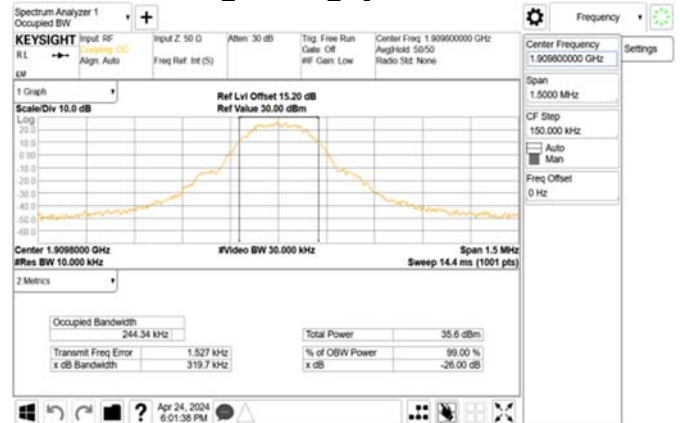
GPMS_1900MHz_HighCH810-1909.8
