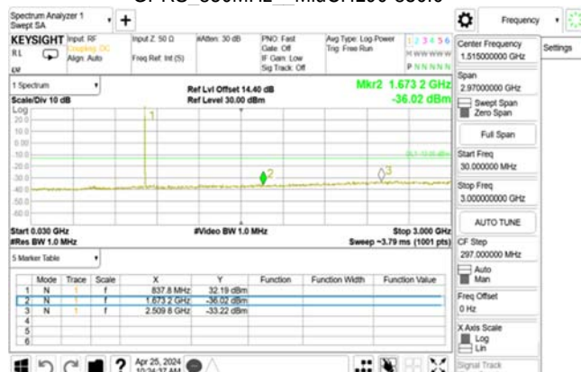
GPRS_850MHz_MidCH190-836.6
