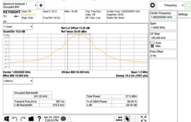
GSM_1900MHz_LowCH512-1850.2
