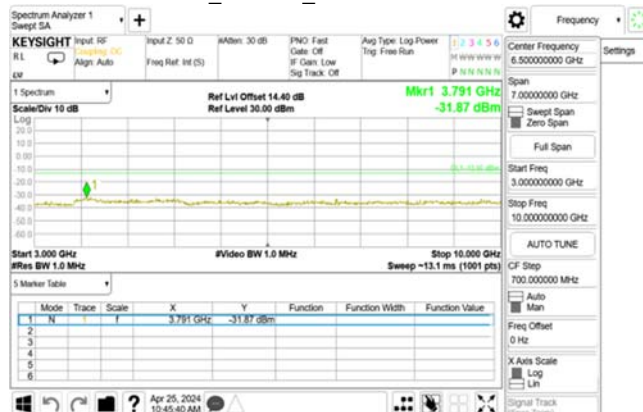
GSM_850MHz_MidCH190-836.6
