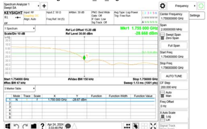
Band Edge WCDMA_B4_HighCH1513-1752.6
