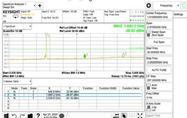
HSUPA_B5_HighCH4233-846.6
