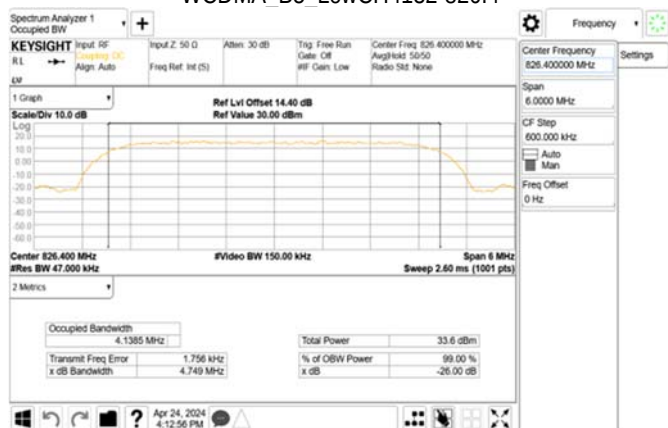
WCDMA_B5_LowCH4132-826.4
