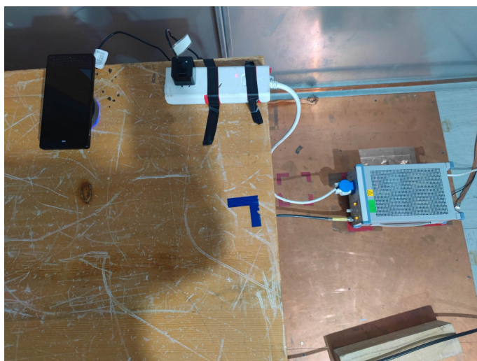
Conducted Emissions Test Setup
