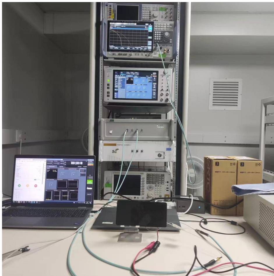
RF Conducted Test setup (GSM/WCDMA/LTE/NR)
