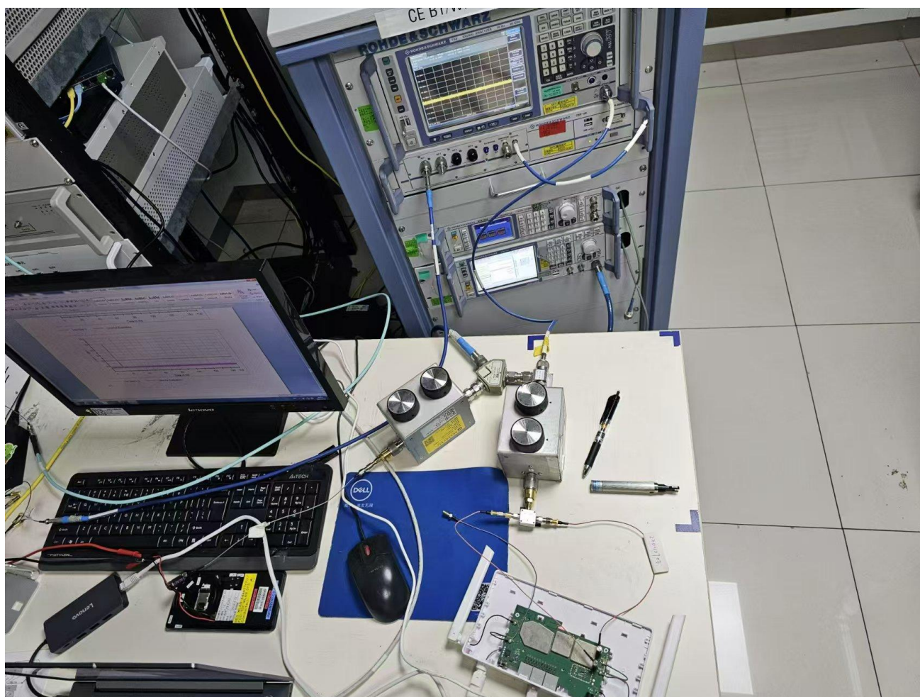
RF Conducted Test setup (DFS)
