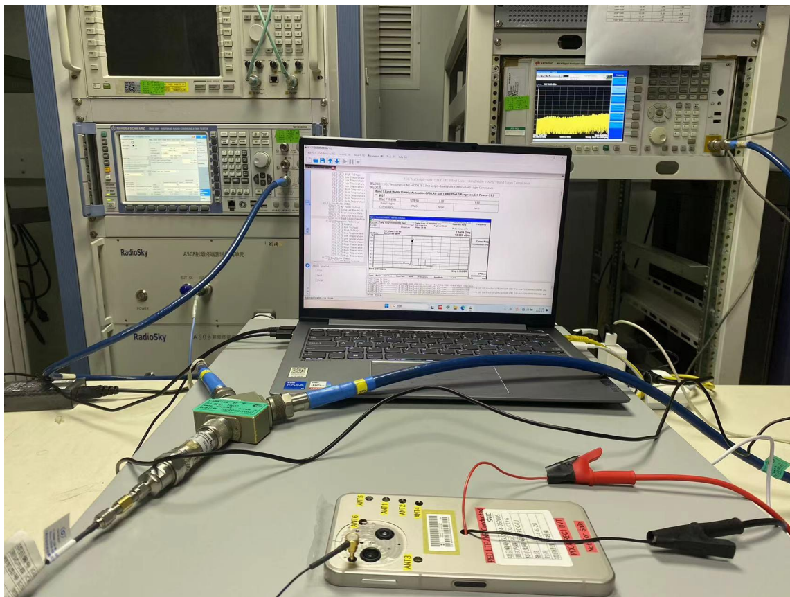
RF Conducted Test setup (GSM/WCDMA/LTE/NR)
