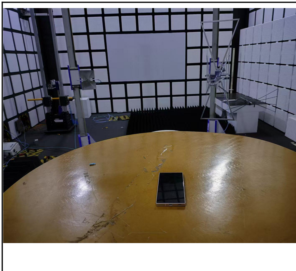
Radiated emission setup photo
