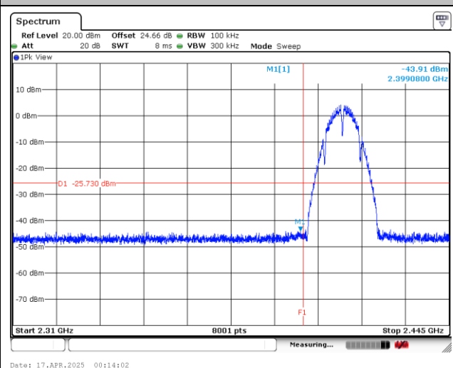
Channel 01 Plot
