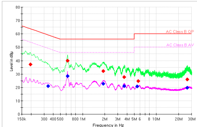
Pic2. Conducted emission L&N Line
