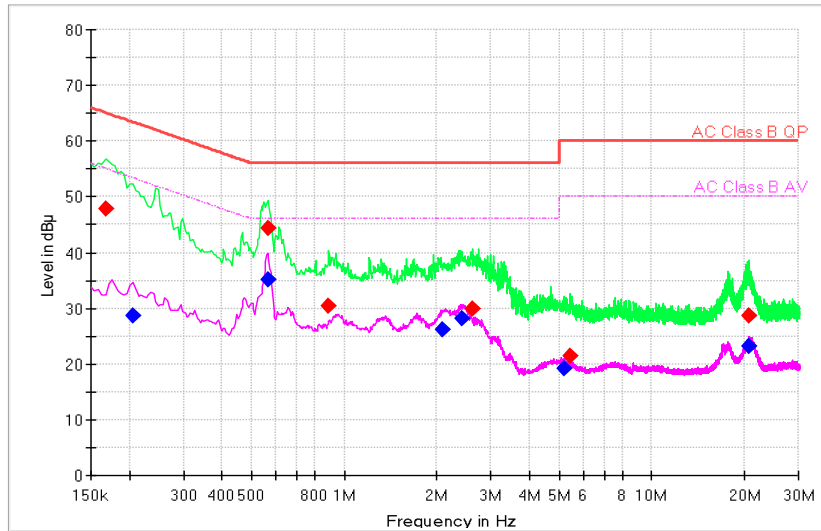
Pic1 Conducted emission L&N Line
