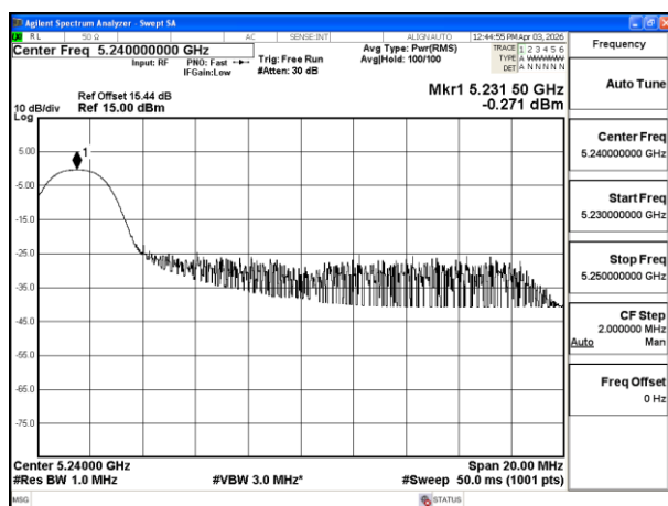
Mode:802.11be EHT20 Tone:26T Frequency:5240MHz Ant:ANT3
