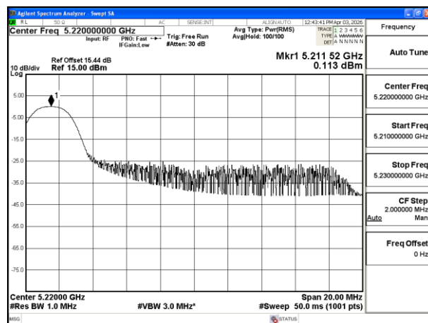
Mode:802.11be EHT20 Tone:26T Frequency:5220MHz Ant:ANT3
