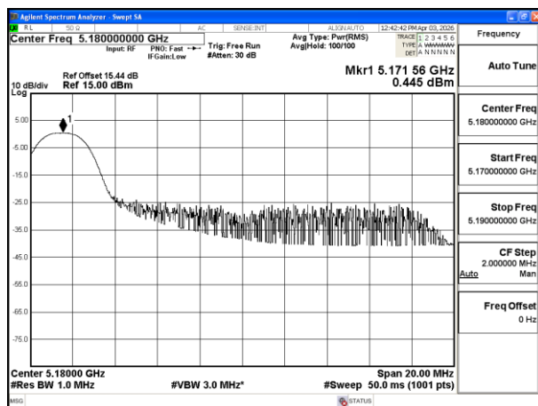
Mode:802.11be EHT20 Tone:26T Frequency:5180MHz Ant:ANT3
