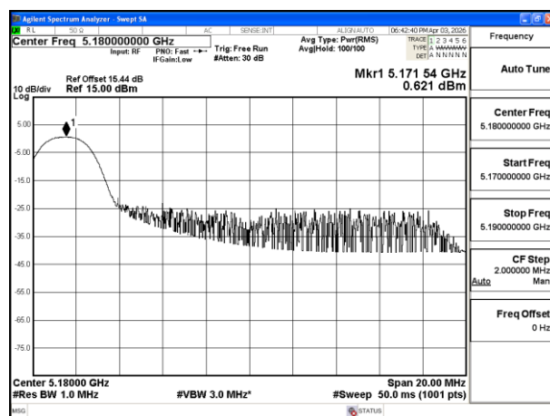
Mode:802.11be EHT20 Tone:26T Frequency:5180MHz Ant:ANT7
