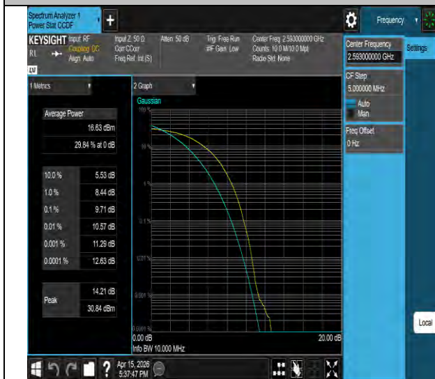
Band41-15MHz-16QAM-40620-75RB#0-PASS
