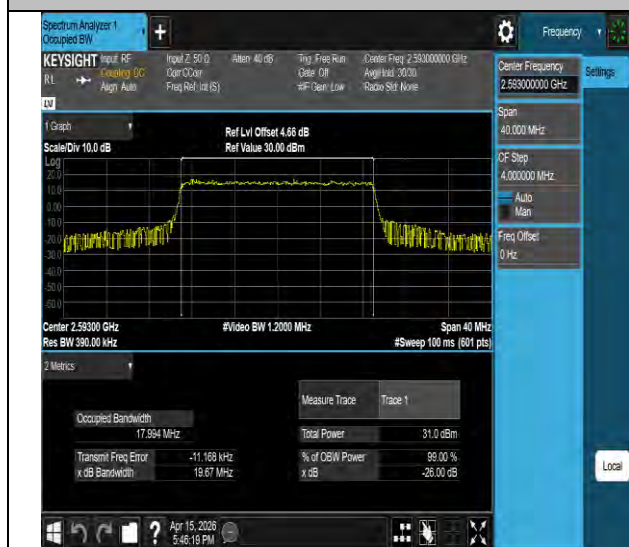
Band41-20MHz-QPSK-40620-100RB#0-PASS
