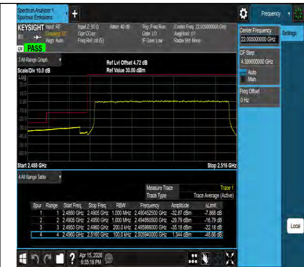
Band41-20MHz-QPSK-39750-100RB#0-PASS
