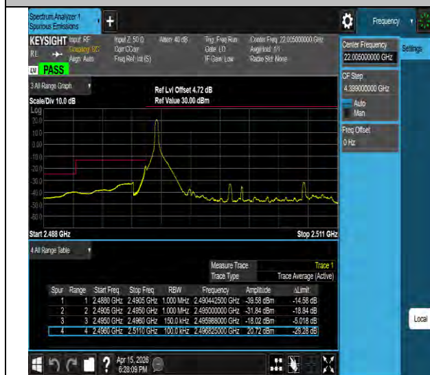
Band41-15MHz-QPSK-39725-1RB#0-PASS
