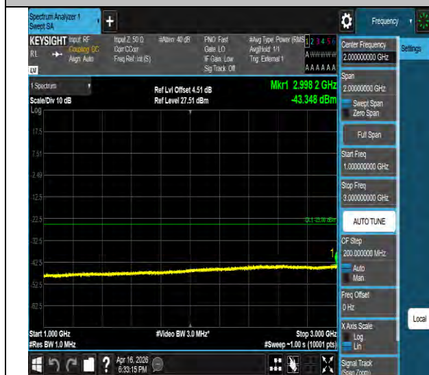
Band41-20MHz-QPSK-40620-1RB#0-1000~3000-PASS
