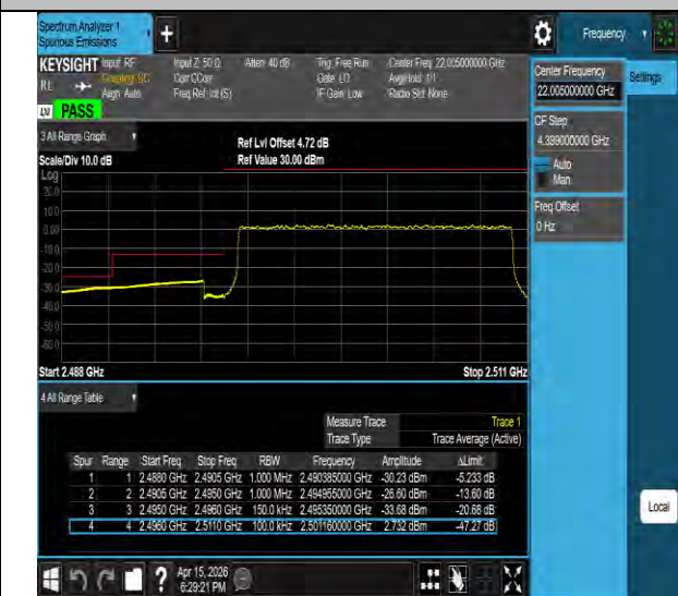
Band41-15MHz-QPSK-39725-75RB#0-PASS
