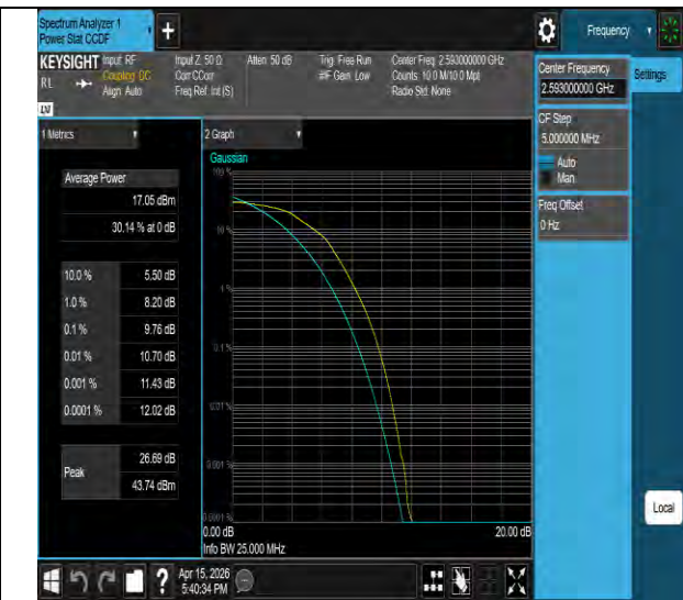
Band41-20MHz-16QAM-40620-100RB#0-PASS
