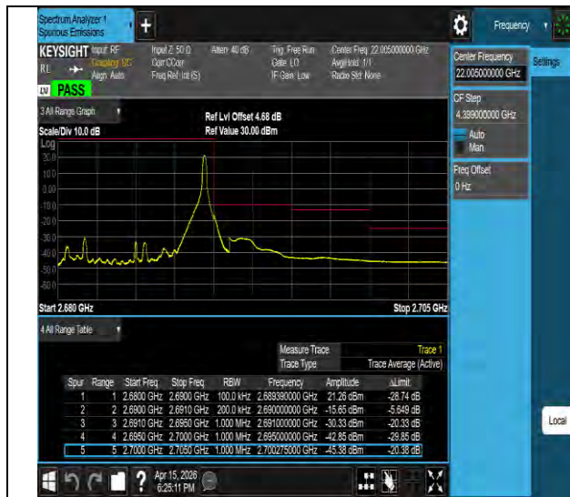
Band41-10MHz-QPSK-41540-1RB#49-PASS
