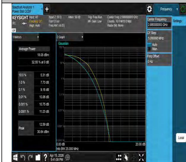
Band41-20MHz-16QAM-41490-100RB#0-PASS
