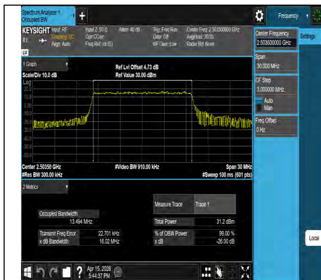
Band41-15MHz-QPSK-39725-75RB#0-PASS
