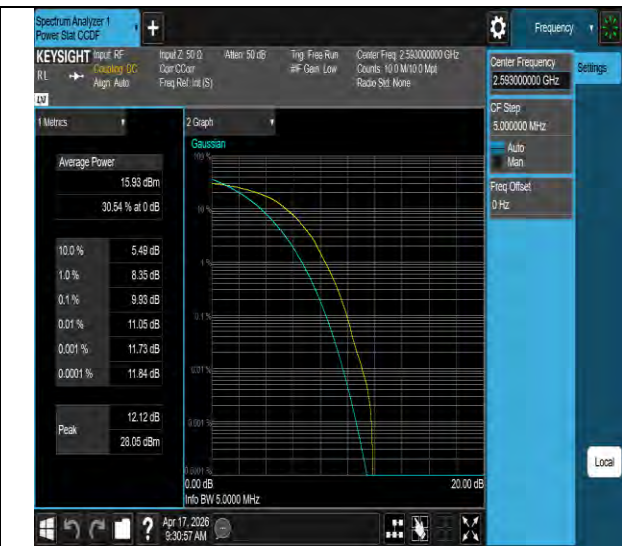
Band41-5MHz-64QAM-40620-25RB#0-PASS
