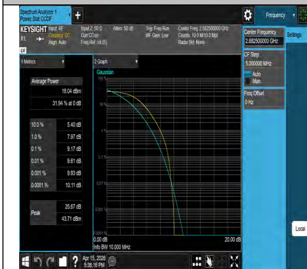
Band41-15MHz-QPSK-41515-75RB#0-PASS
