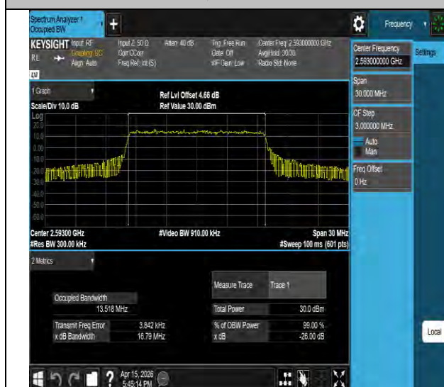
Band41-15MHz-16QAM-40620-75RB#0-PASS
