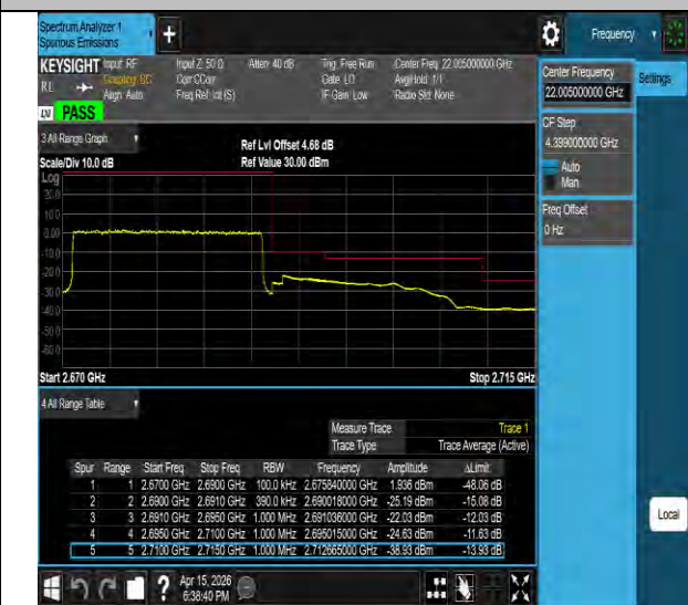
Band41-20MHz-QPSK-41490-100RB#0-PASS
