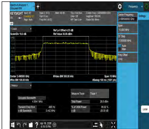
Band41-5MHz-64QAM-39675-25RB#0-PASS
