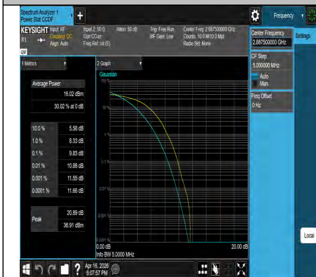
Band41-5MHz-64QAM-41565-25RB#0-PASS
