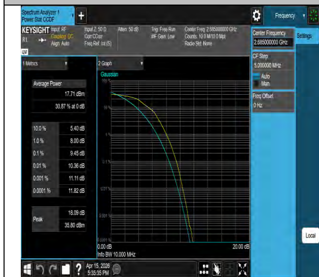
Band41-10MHz-16QAM-41540-50RB#0-PASS
