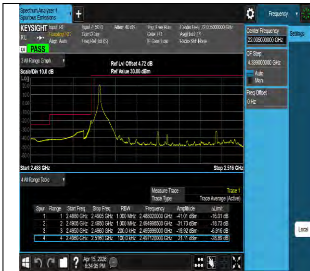
Band41-20MHz-QPSK-39750-1RB#0-PASS
