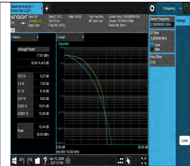
Band41-15MHz-QPSK-40620-75RB#0-PASS
