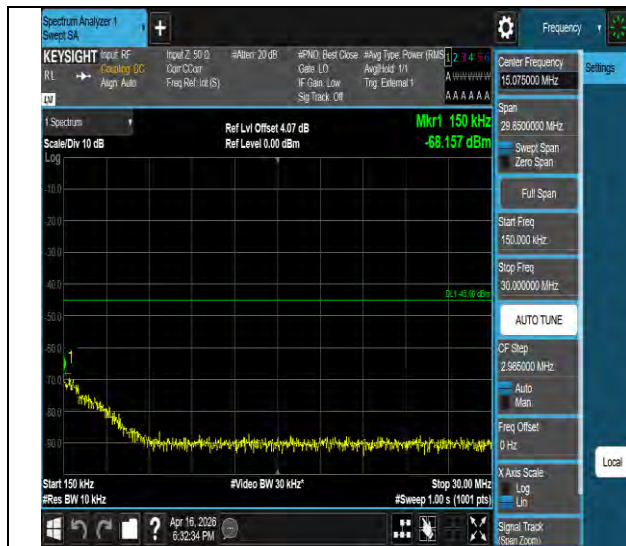
Band41-20MHz-QPSK-40620-1RB#0-0.15~30-PASS
