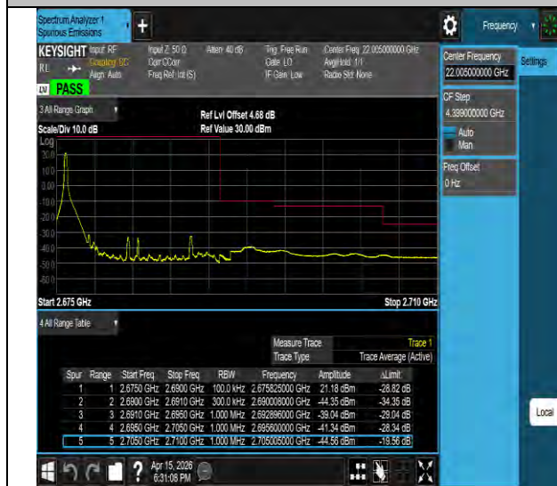
Band41-15MHz-QPSK-41515-1RB#0-PASS
