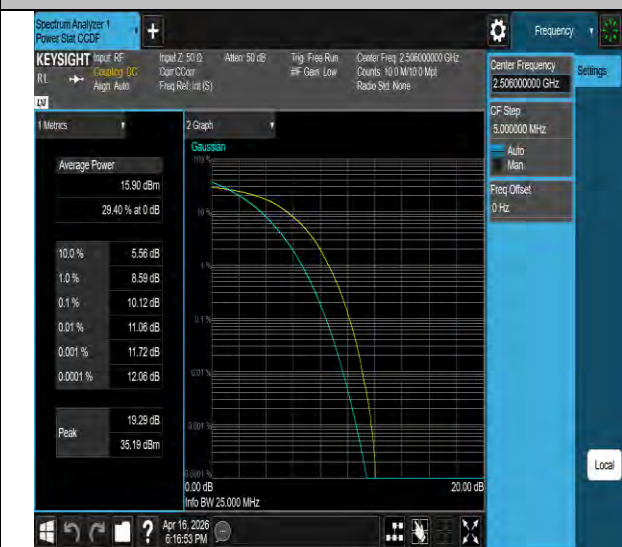
Band41-20MHz-64QAM-39750-100RB#0-PASS
