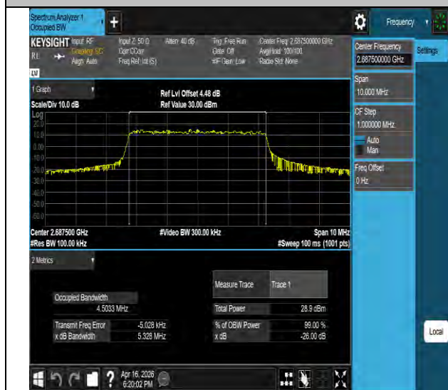
Band41-5MHz-64QAM-41565-25RB#0-PASS
