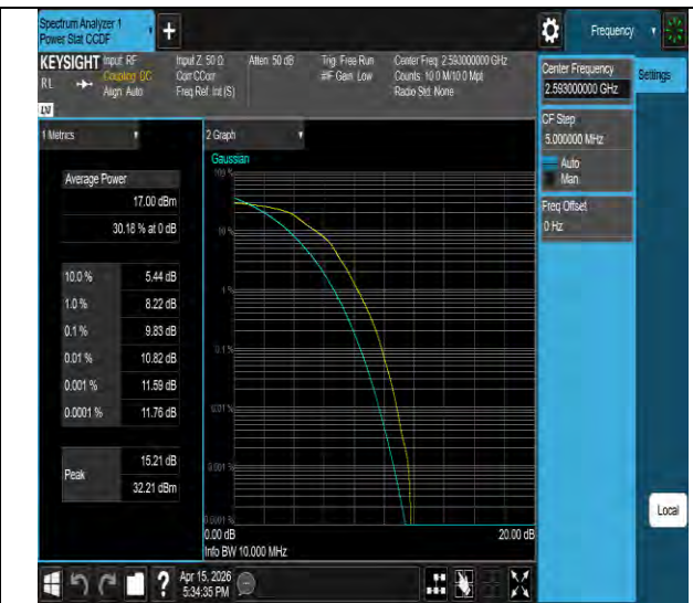
Band41-10MHz-16QAM-40620-50RB#0-PASS
