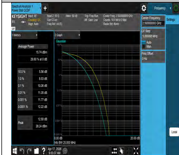
Band41-20MHz-64QAM-40620-100RB#0-PASS
