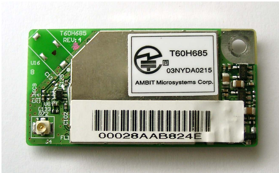
WLAN module Side A (with shield)
