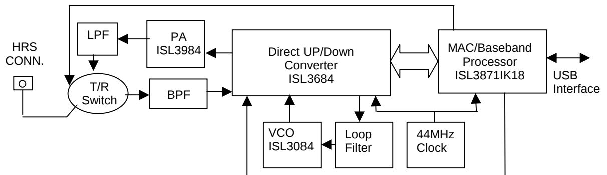
Figure 1. System block diagram of T60H685.00
