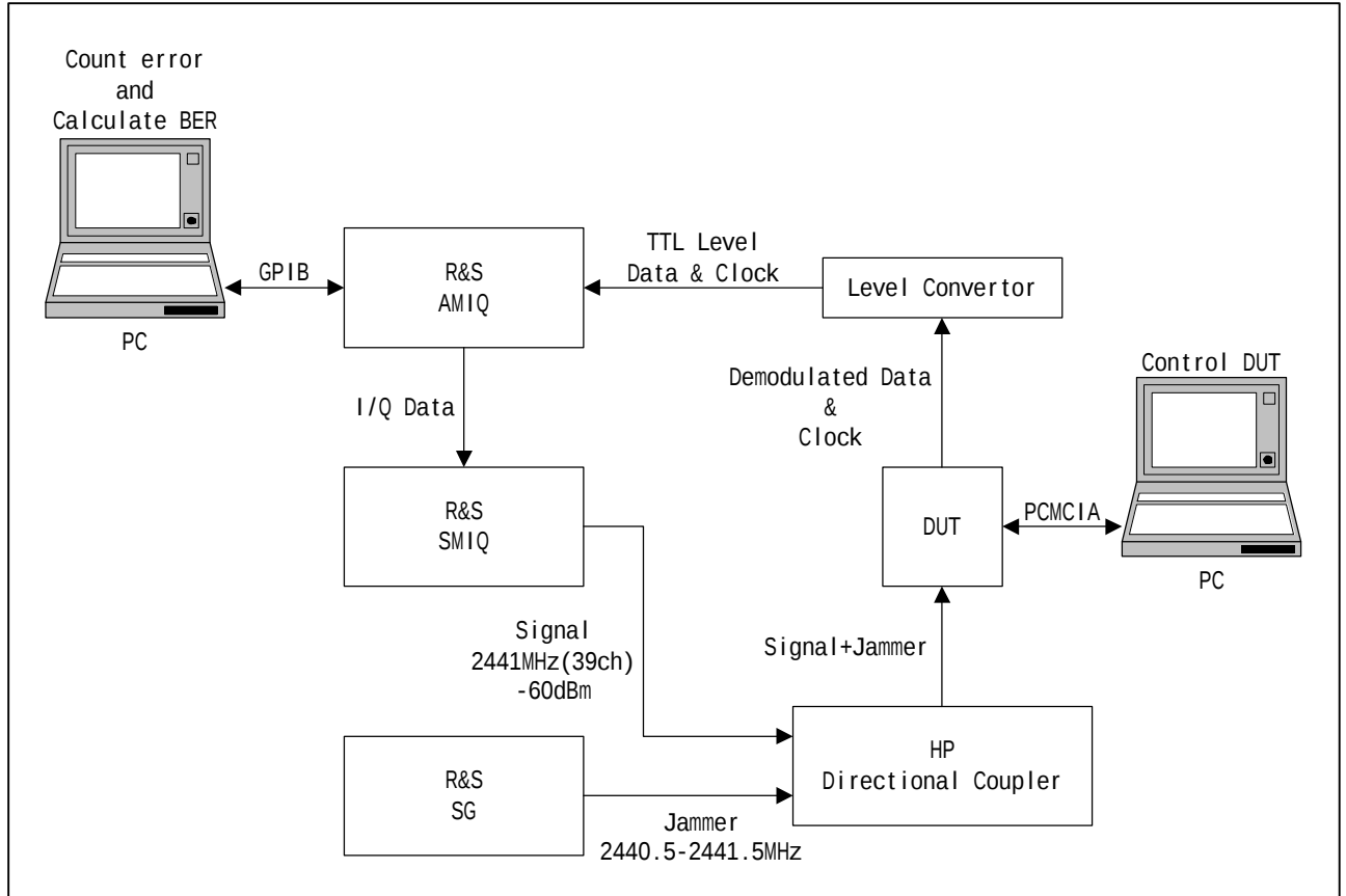
Fig. 1 Measurement Arrangement and Equipment List
