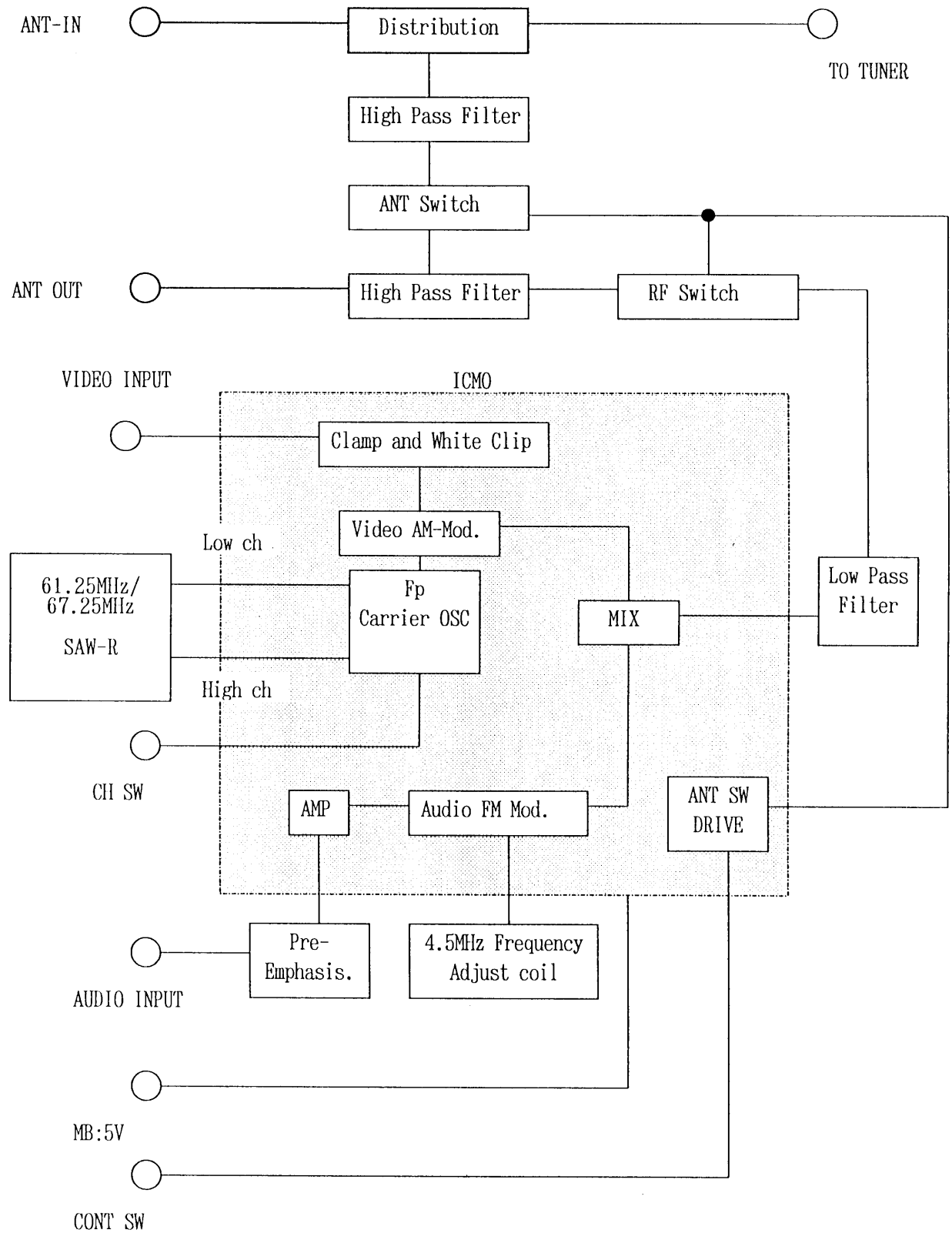
[ RF Modulator Section block Diagram ]
