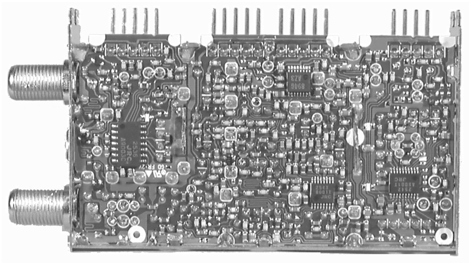
Solder side of Tuner/RF Converter PWB of Model VC-H998U Parts Code : VTUNJH3091U28
