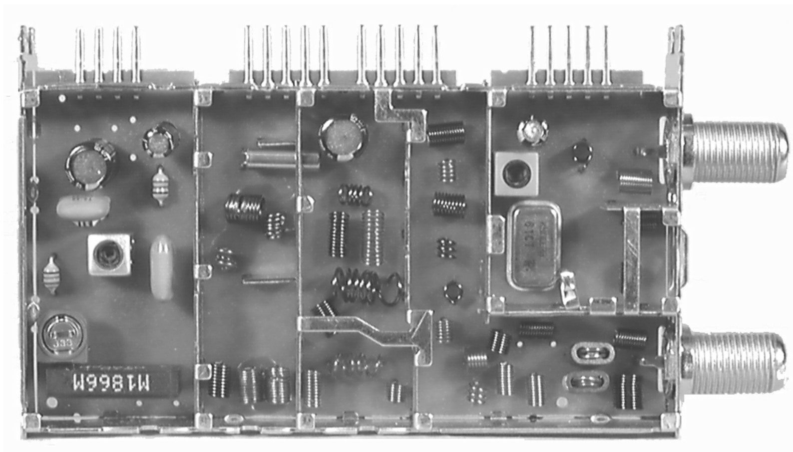
Component Side of Tuner/RF Converter PWB of Model VC-H998U Parts Code : VTUNJH3091U28
