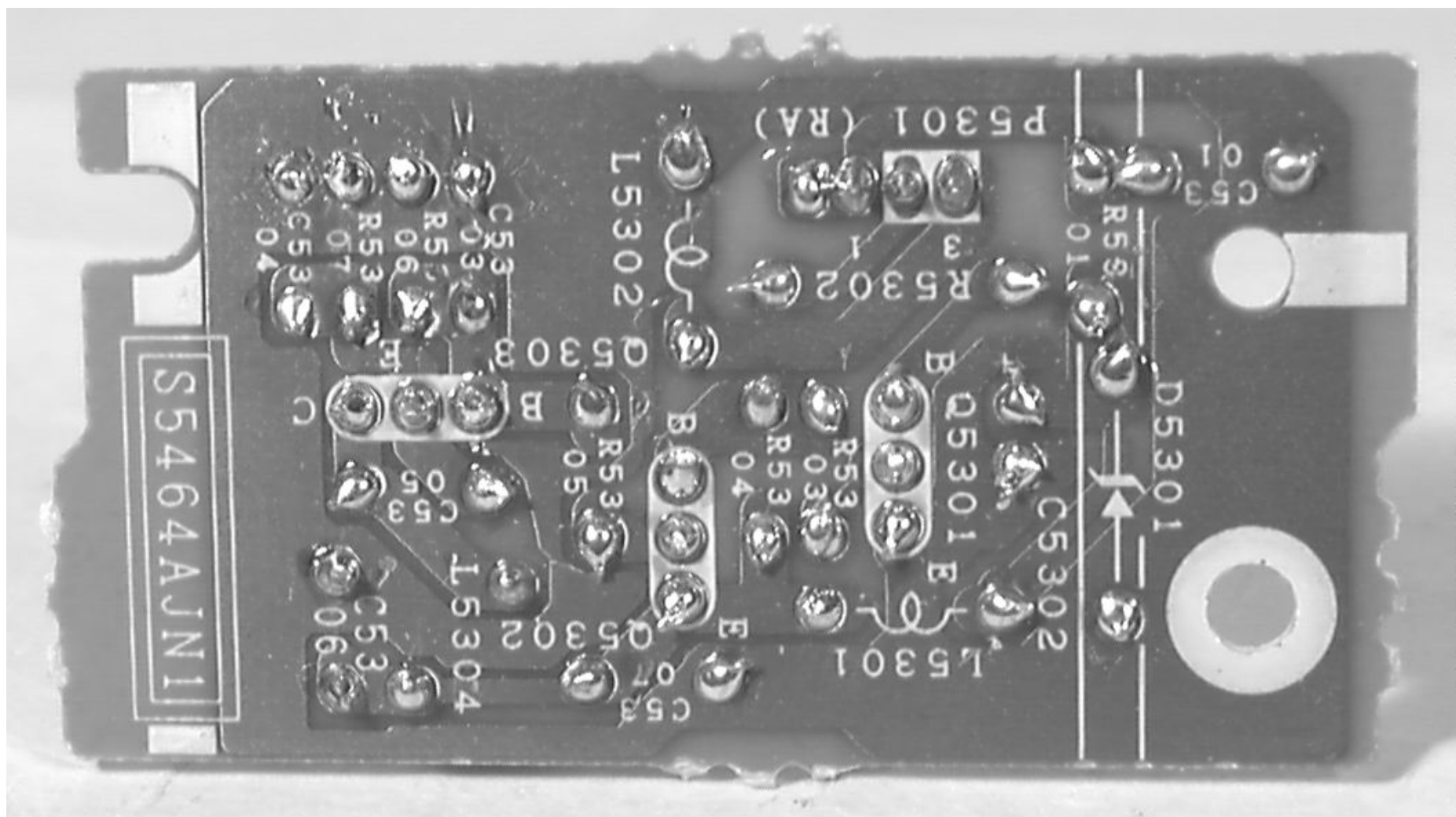
Locator PWB (Solder Side)
