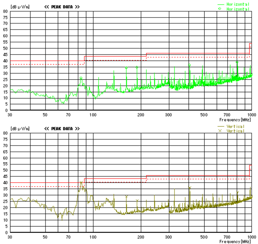
Figure 31 Tx_Horizontally Place
