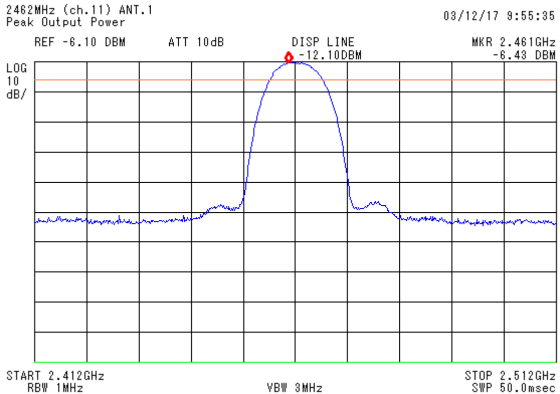
figure 11 2462 MHz_0a (channel 11)
