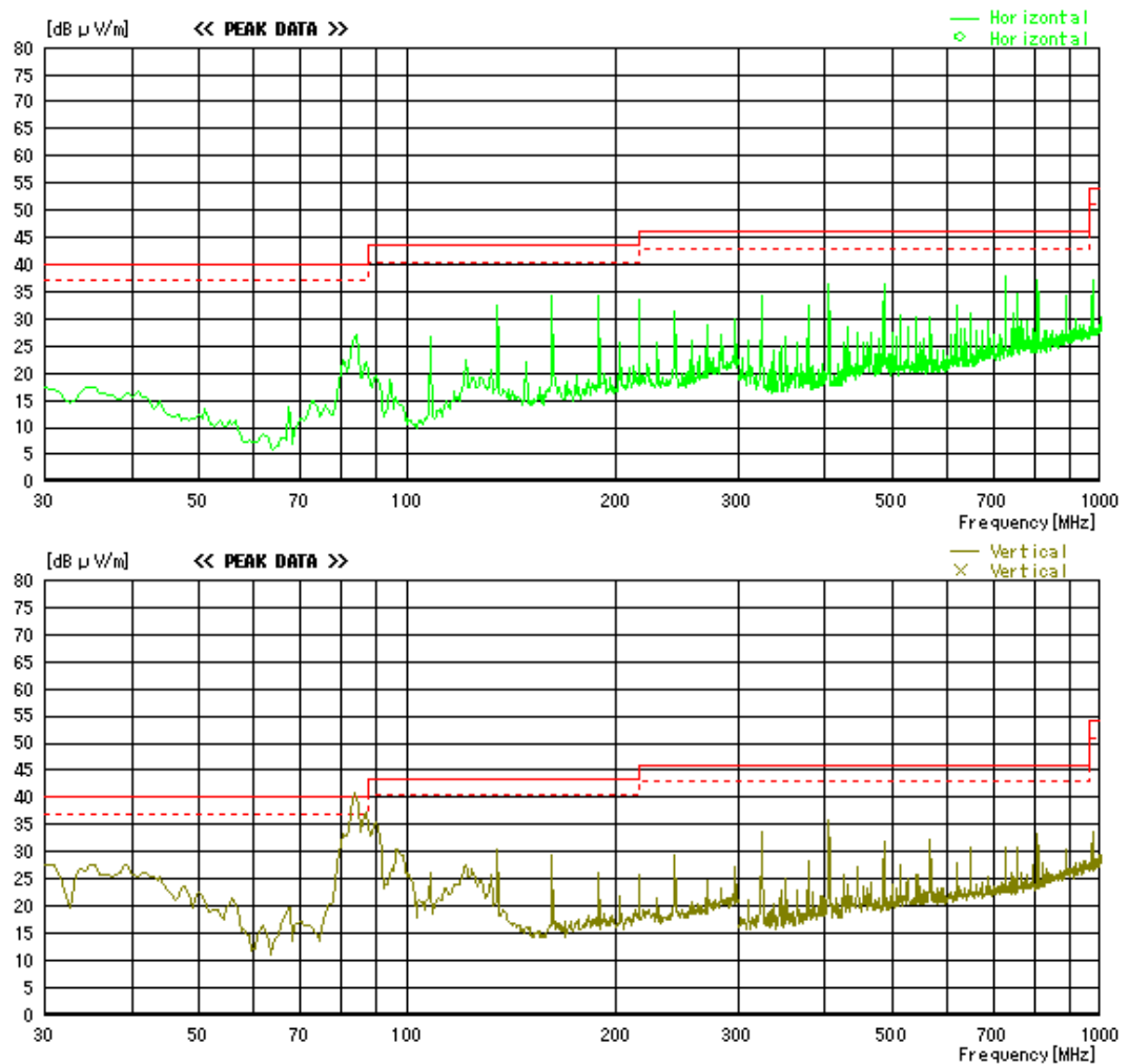
Figure 29 Rx_Horizontally Place
