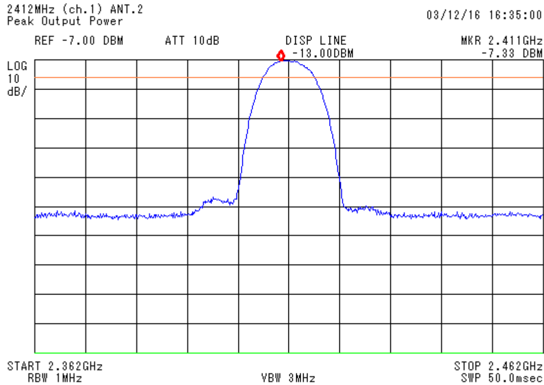
figure 8 2412 MHz_4a (channel 1)
