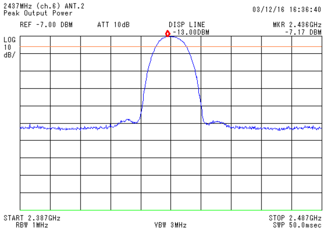
figure 10 2437 MHz_4a (channel 6)
