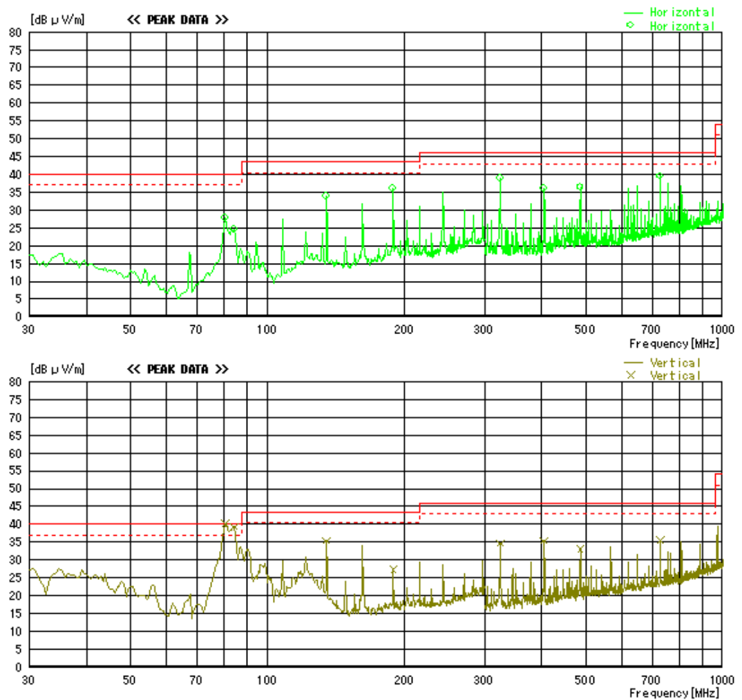
Figure 30 Rx_Vertically Place
