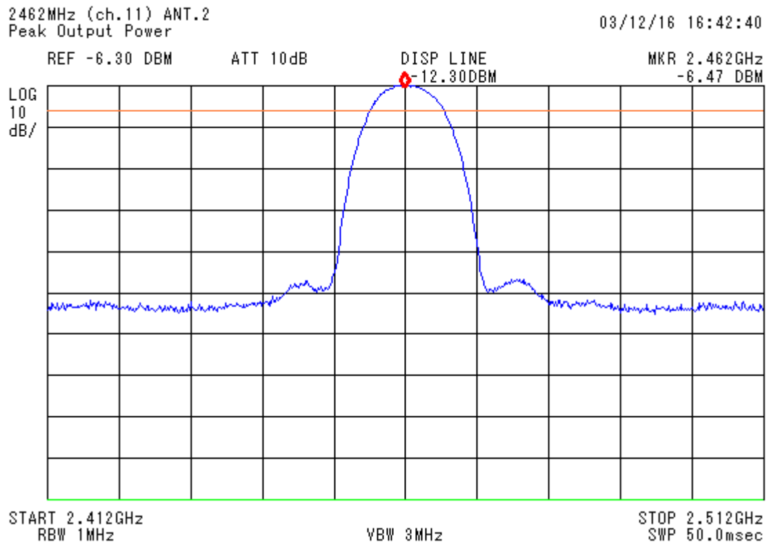
figure 12 2462 MHz_4a (channel 11)
