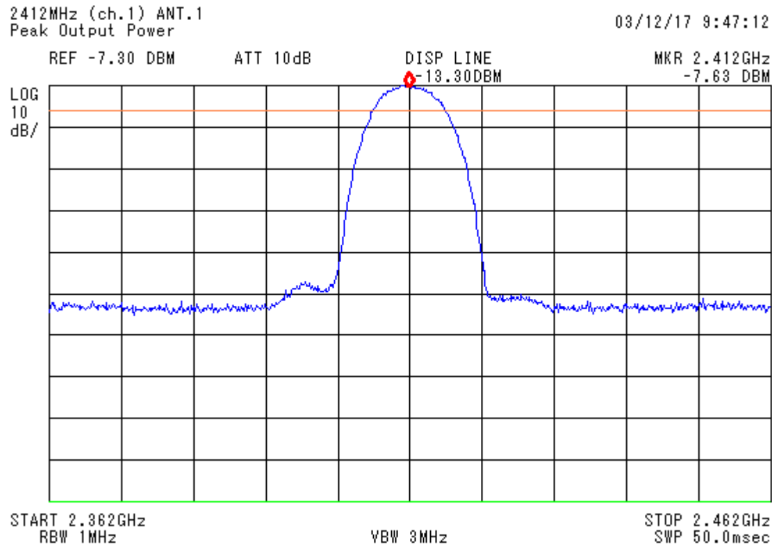
figure 7 2412 MHz_0a (channel 1)
