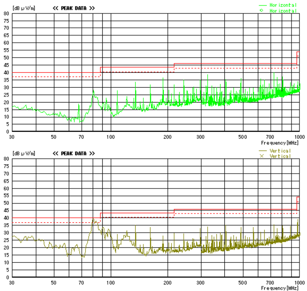
Figure 32 Tx_Vertically Place
