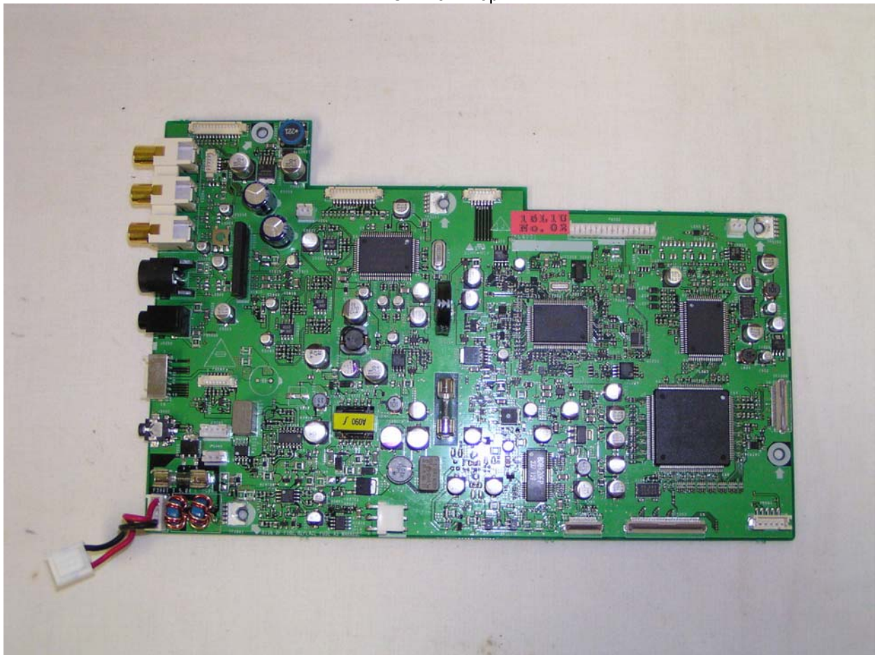
PCB Main Bottom
