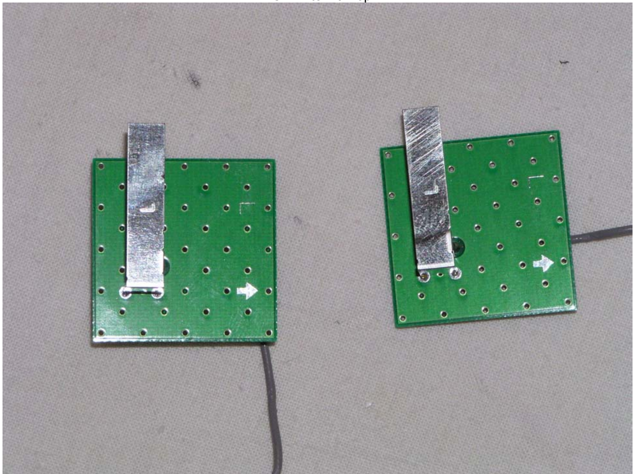
PCB Antenna Bottom
