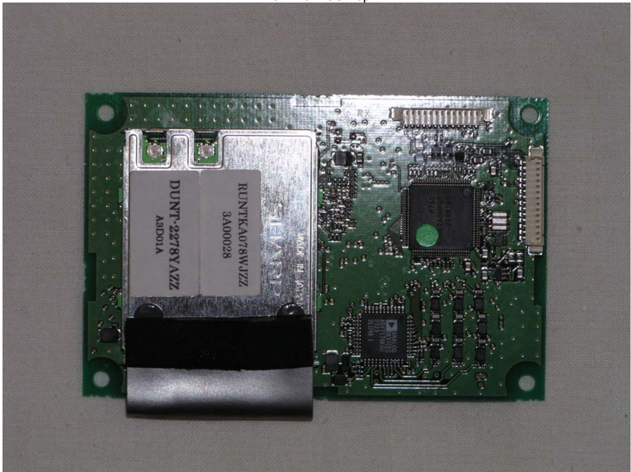
PCB Main SS Top - plate removed
