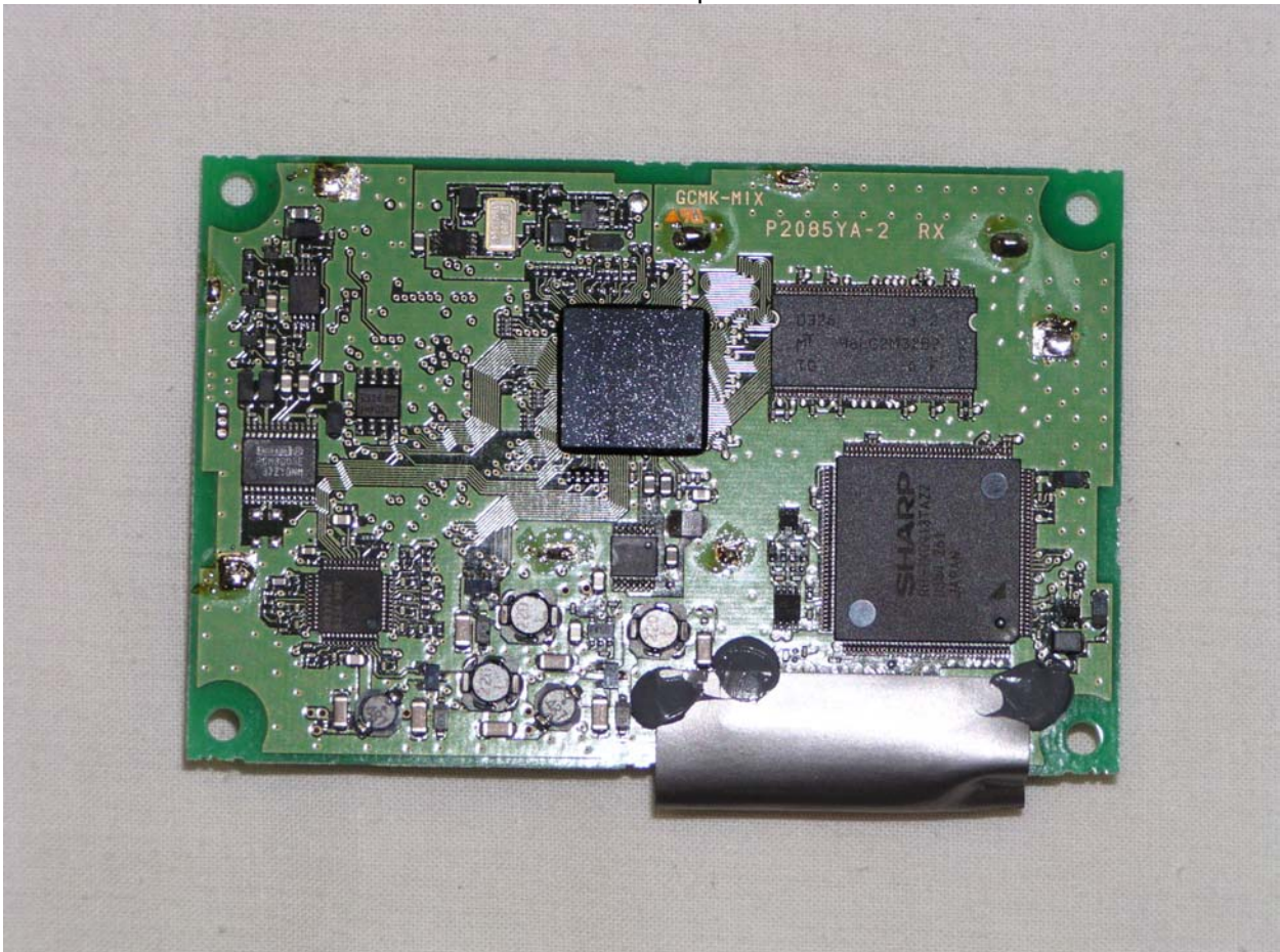
PCB Main SS Bottom - plate removed
