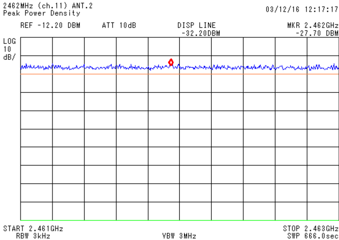
figure 28 Power Density, Tx on channel 11_4a
