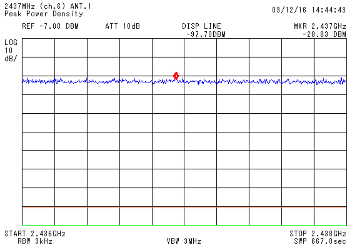
figure 25 Power Density, Tx on channel 6_0a
