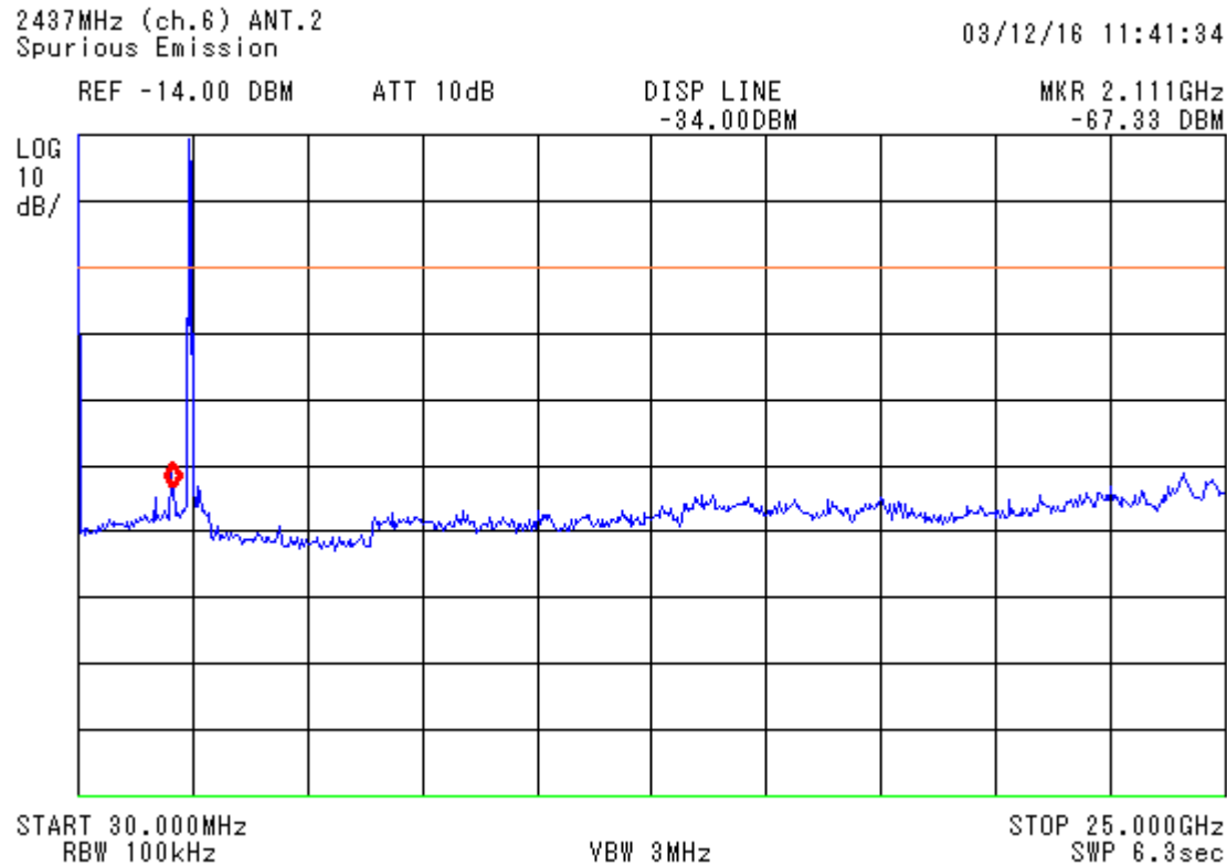
figure 20 Spurious RF conducted emission, Tx on 2437 MHz_4a
