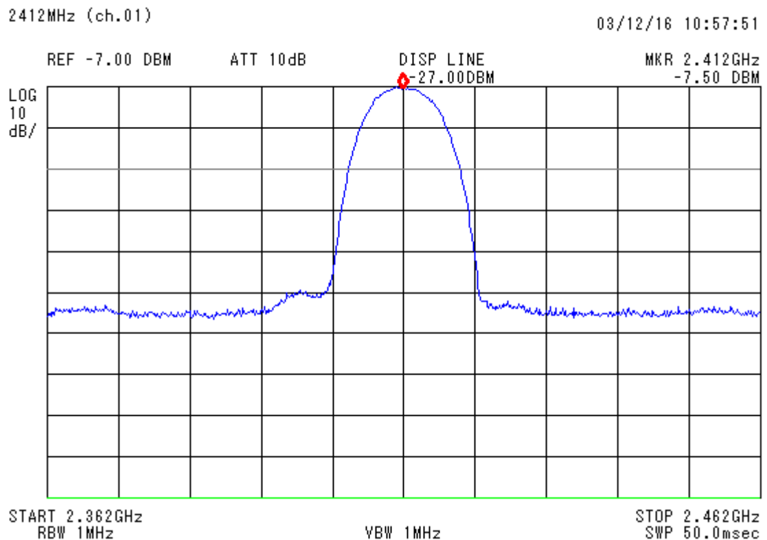
figure 8 2412 MHz_4a (channel 1)
