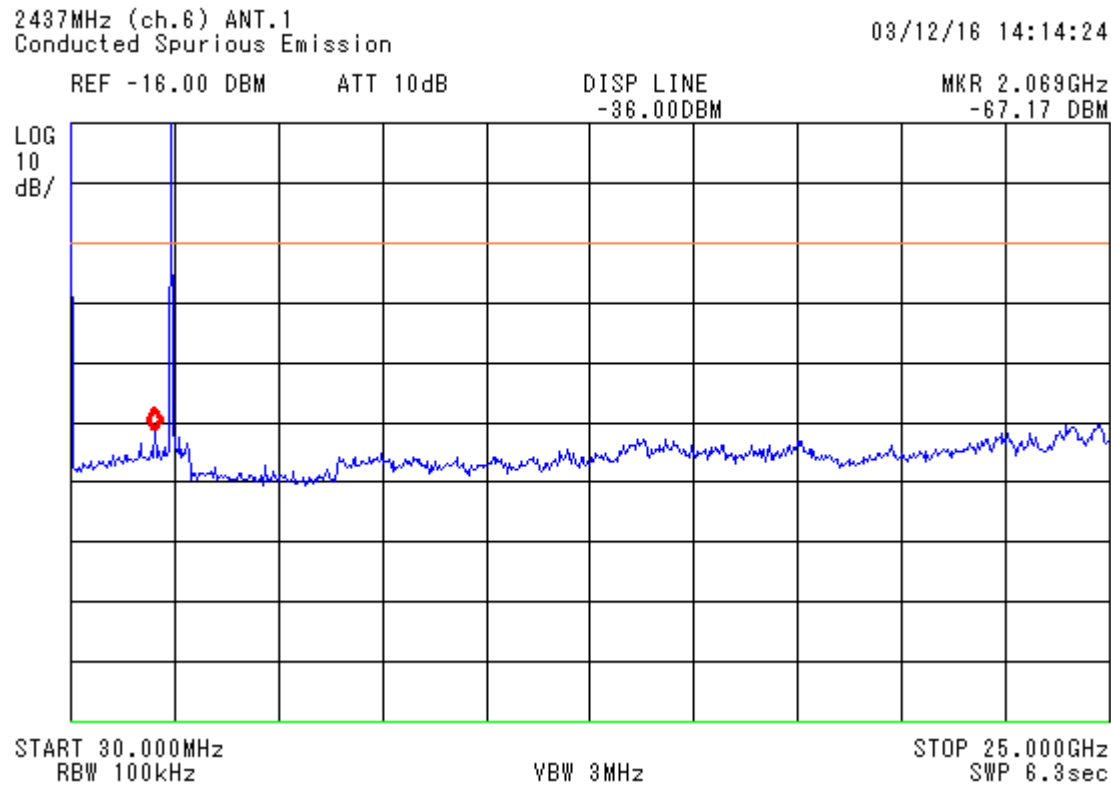
figure 19 Spurious RF conducted emission, Tx on 2437 MHz_0a
