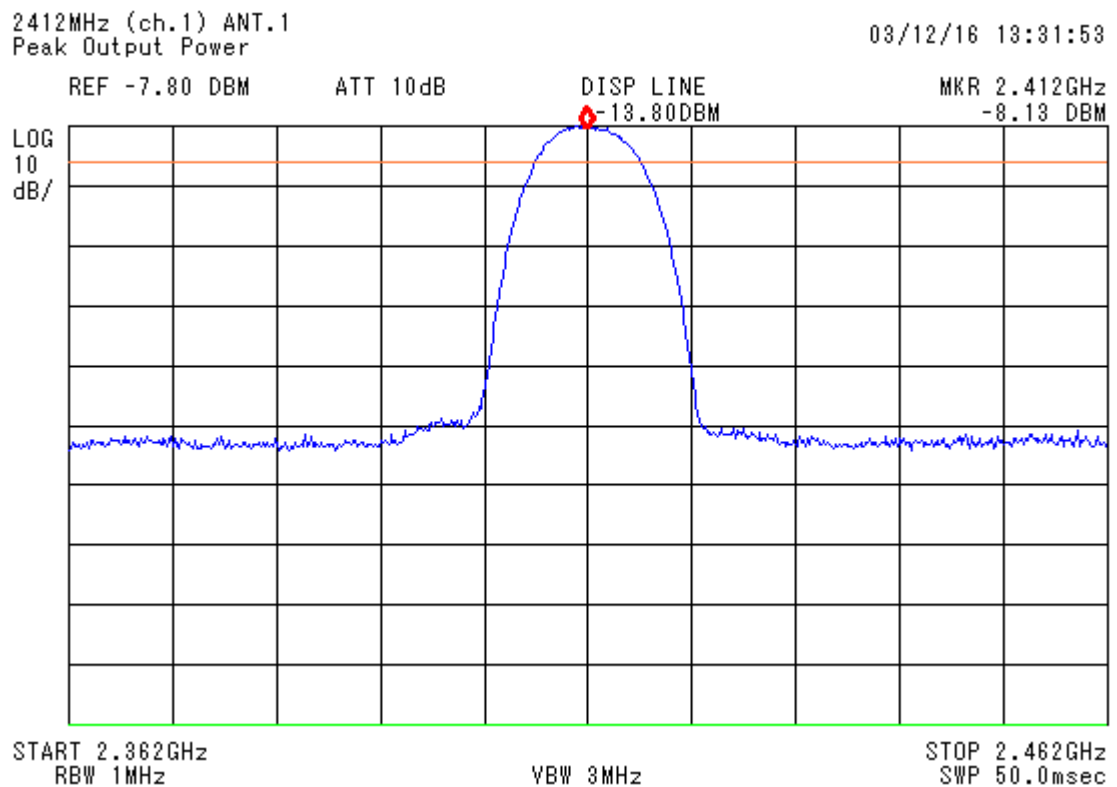
figure 7 2412 MHz_0a (channel 1)
