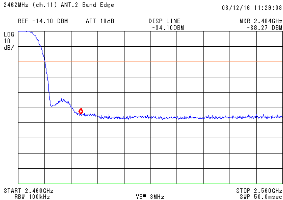
figure 16 Band Edge High frequency side _4a
