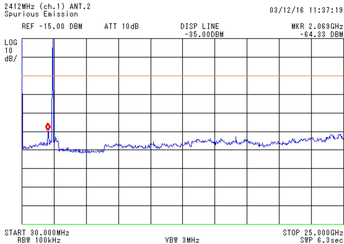
figure 18 Spurious RF conducted emission, Tx on 2412 MHz_4a
