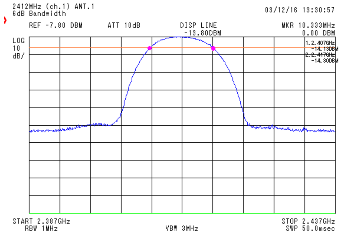
figure 1 6dB Bandwidth fc = 2412 MHz_0a
