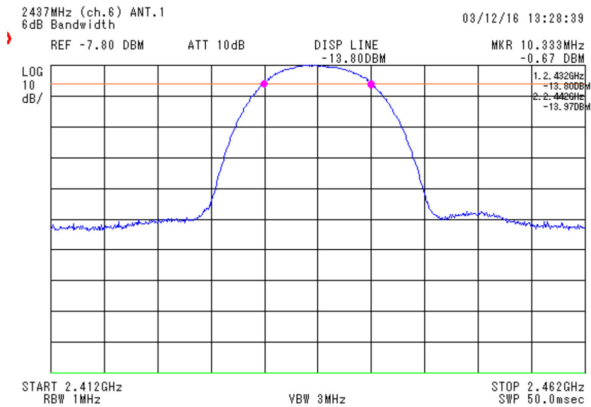
figure 3 6dB Bandwidth fc = 2437 MHz_0a
