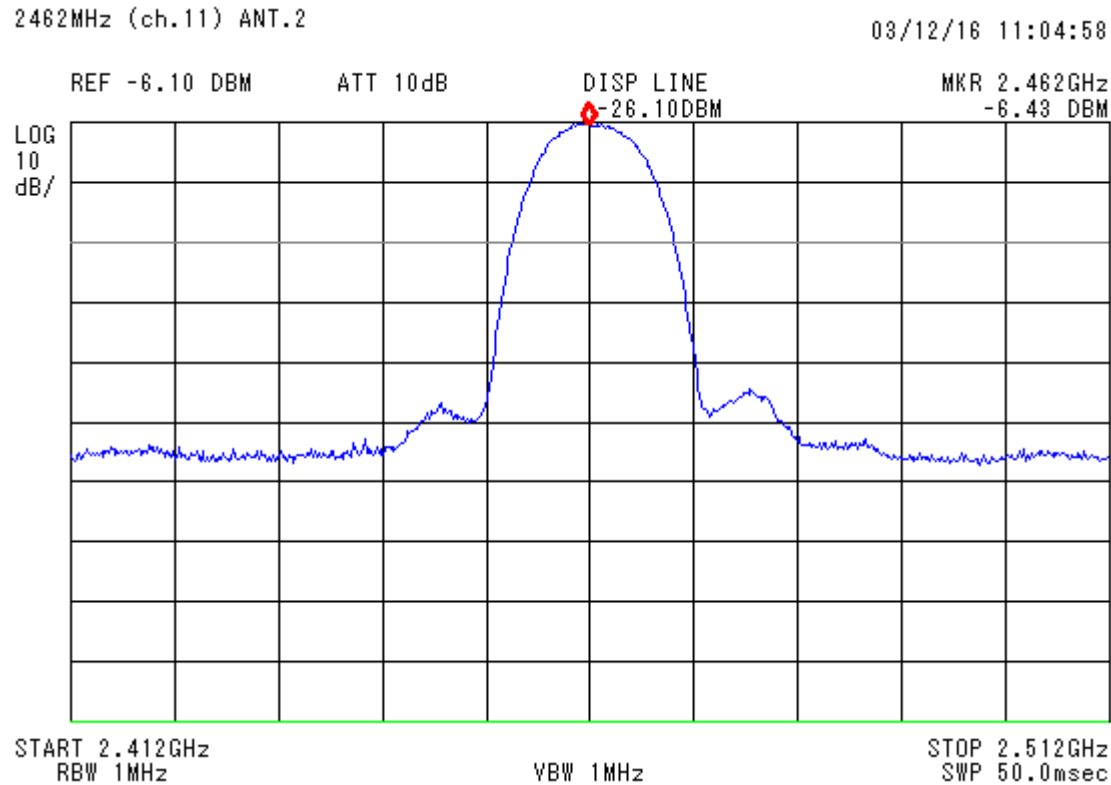
figure 12 2462 MHz_4a (channel 11)
