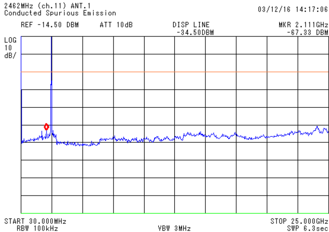
figure 21 Spurious RF conducted emission, Tx on 2462 MHz_0a
