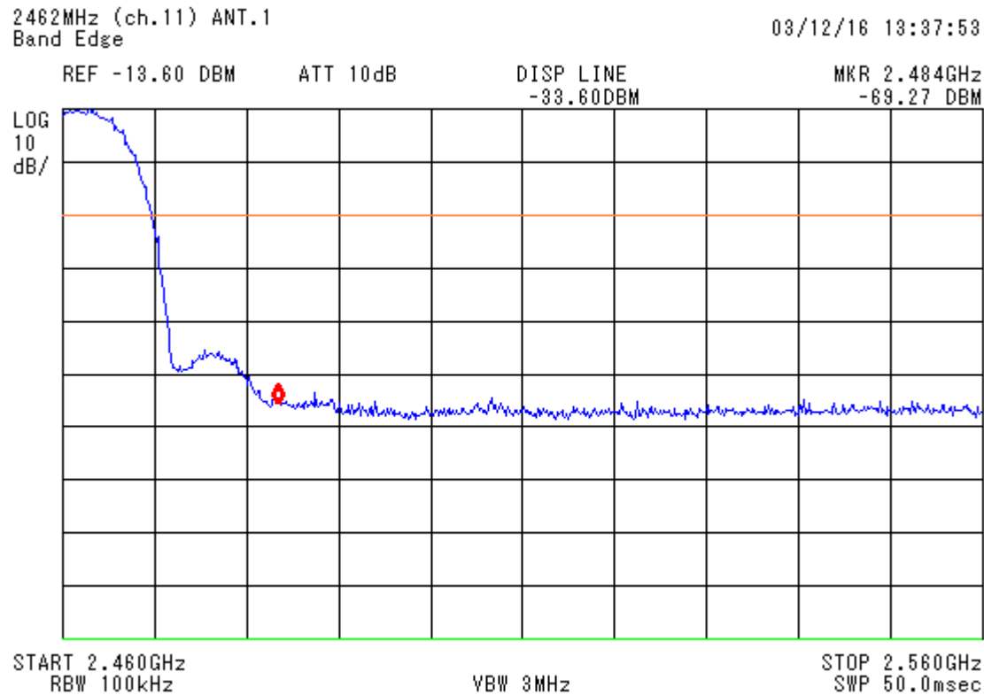
figure 15 Band Edge High frequency side _0a
