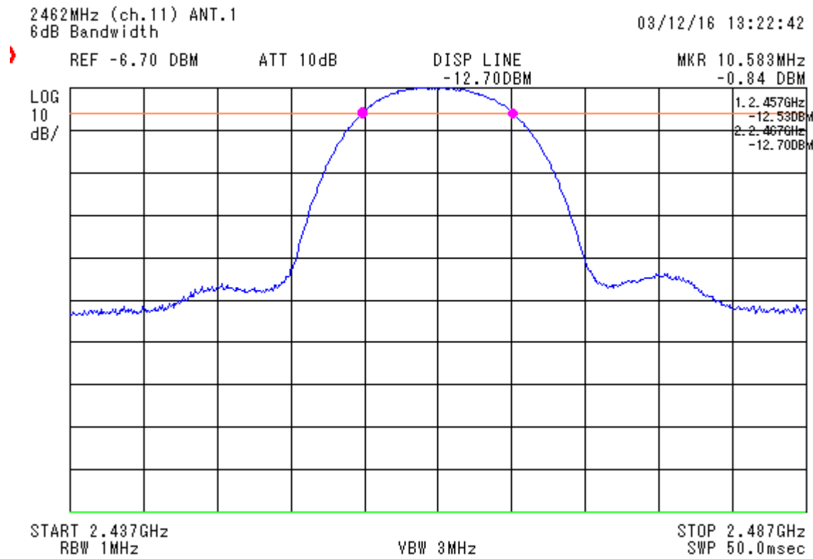
figure 5 6dB Bandwidth fc = 2462 MHz_0a
