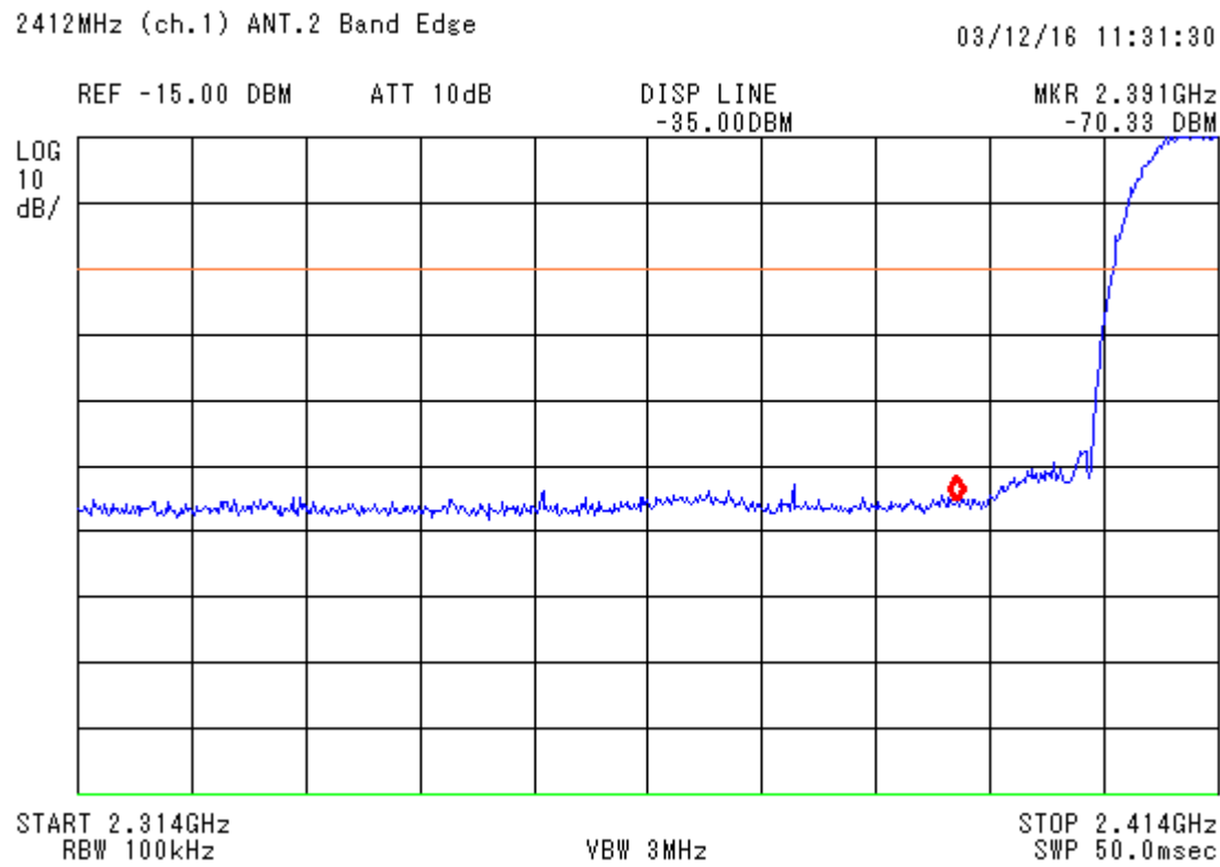
figure 14 Band Edge Low frequency side _4a
