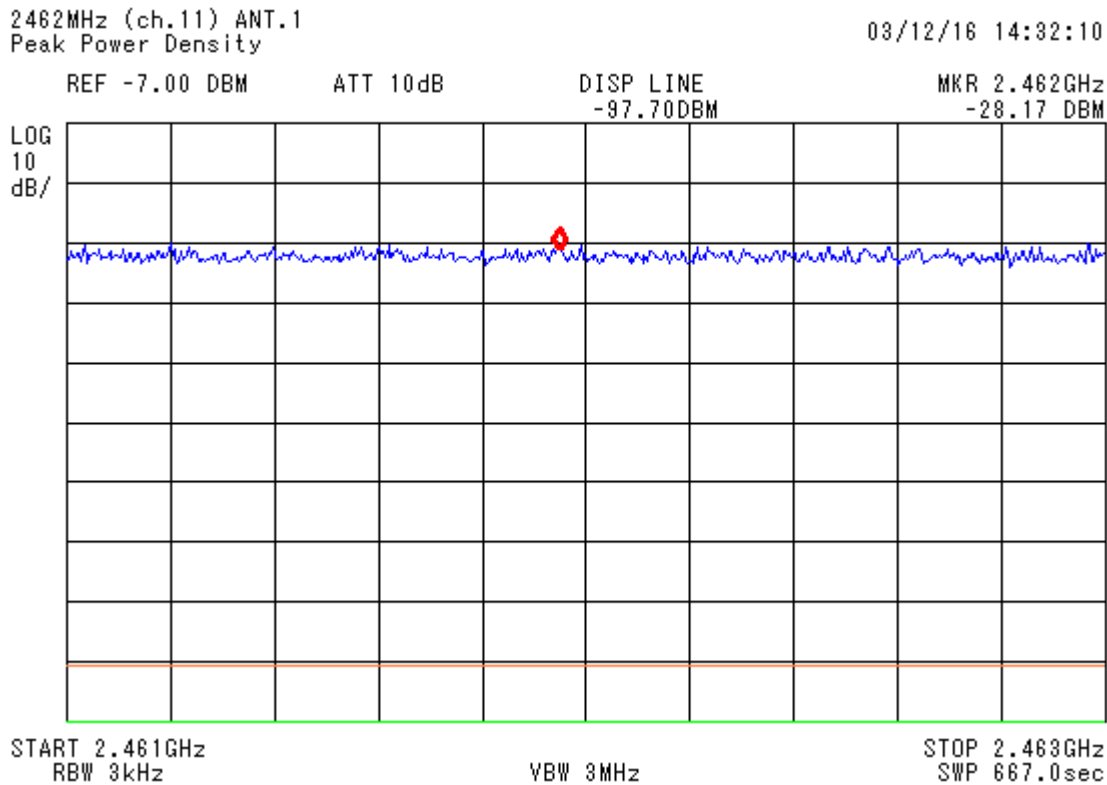
figure 27 Power Density, Tx on channel 11_0a
