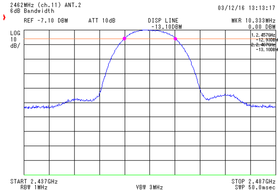
figure 6 6dB Bandwidth fc = 2462 MHz_4a
