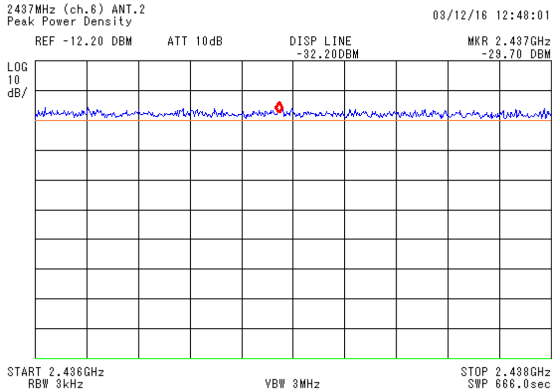
figure 26 Power Density, Tx on channel 6_4a
