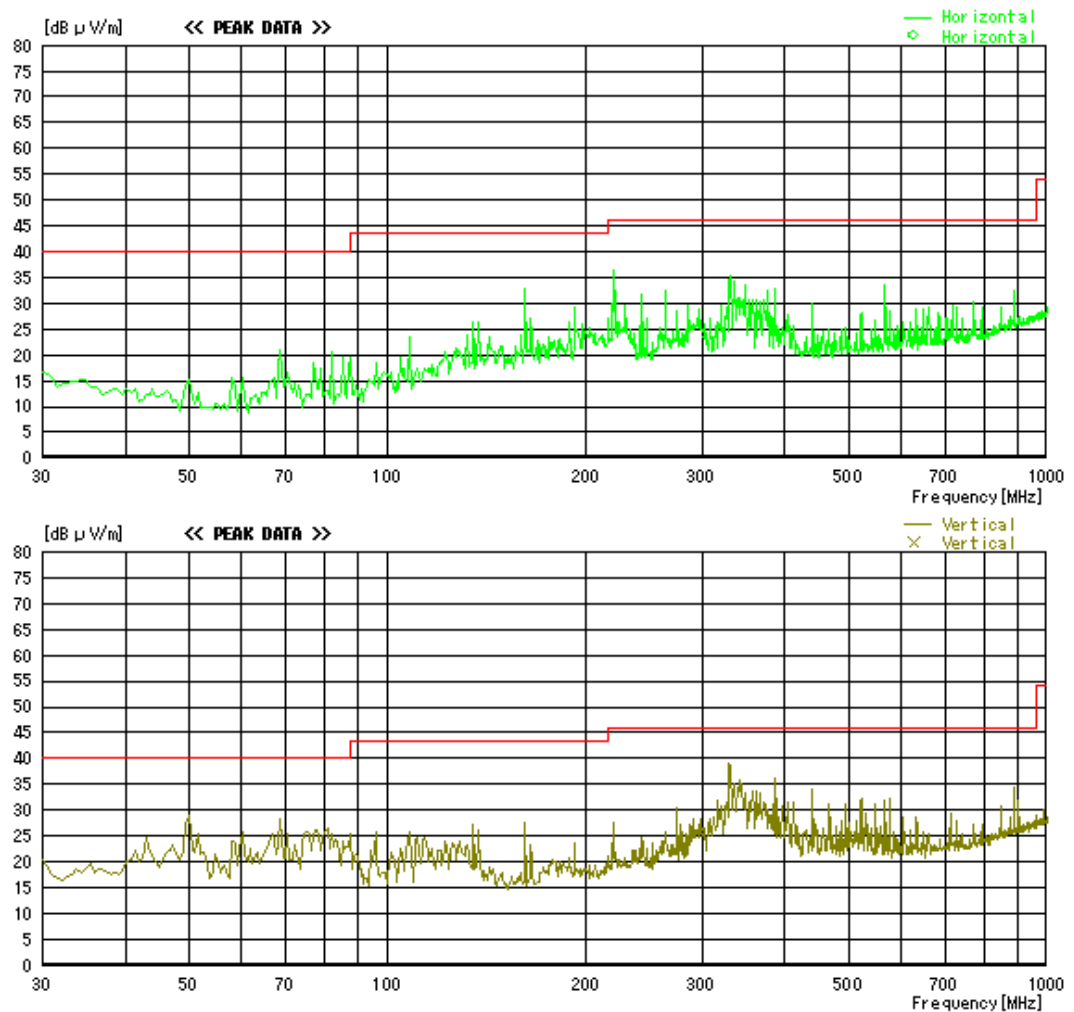
Figure 29 Rx
