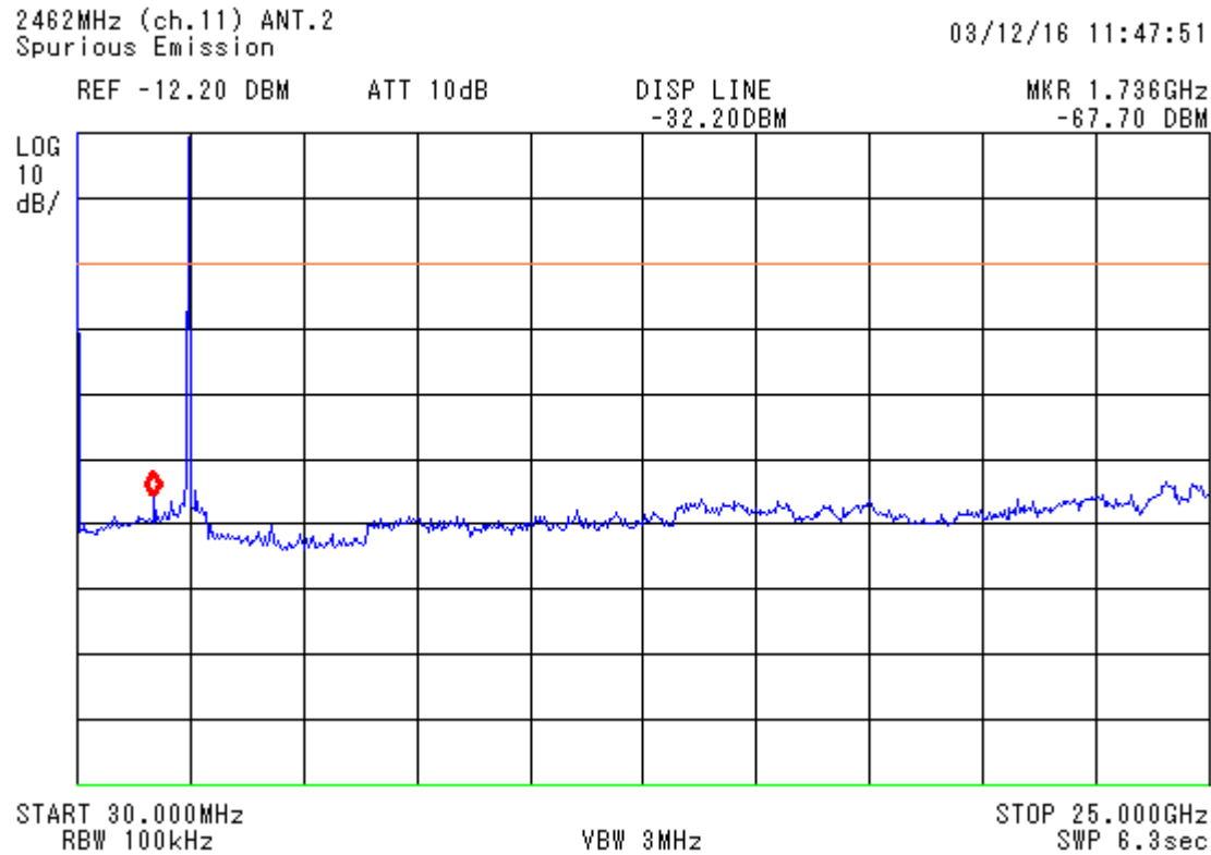
figure 22 Spurious RF conducted emission, Tx on 2462 MHz_4a
