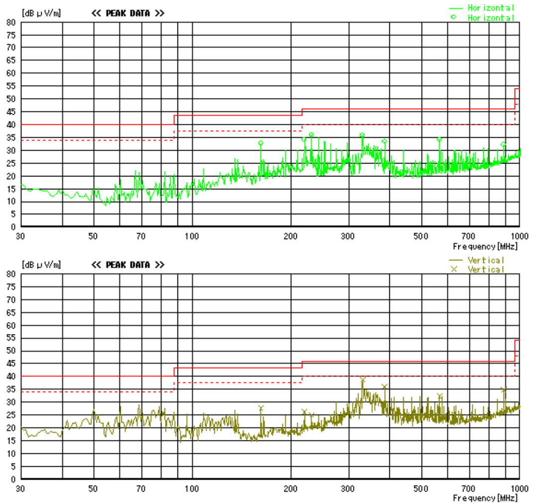
Figure 30 Tx
