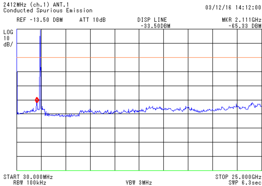
figure 17 Spurious RF conducted emission, Tx on 2412 MHz_0a
