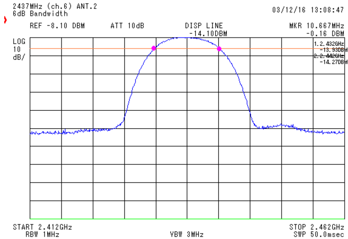
figure 4 6dB Bandwidth fc = 2437 MHz_4a
