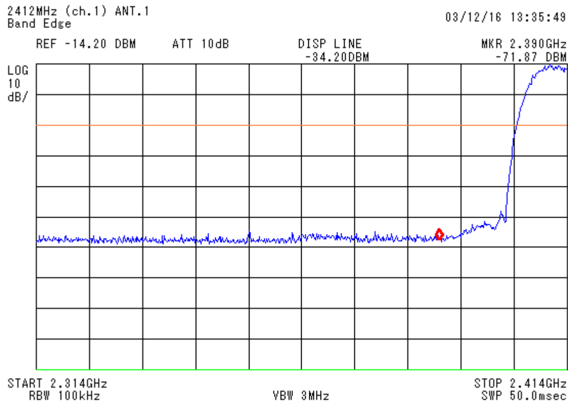
figure 13 Band Edge Low frequency side _0a
