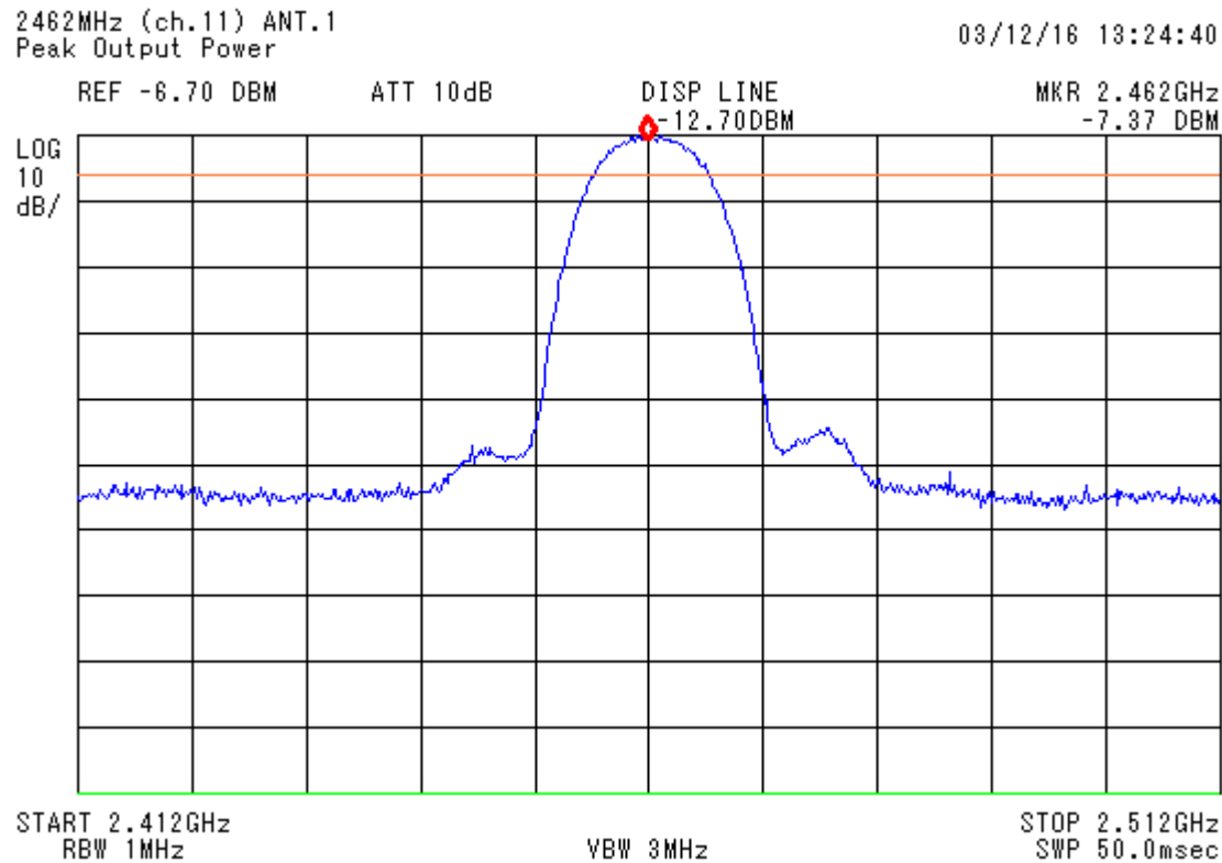
figure 11 2462 MHz_0a (channel 11)
