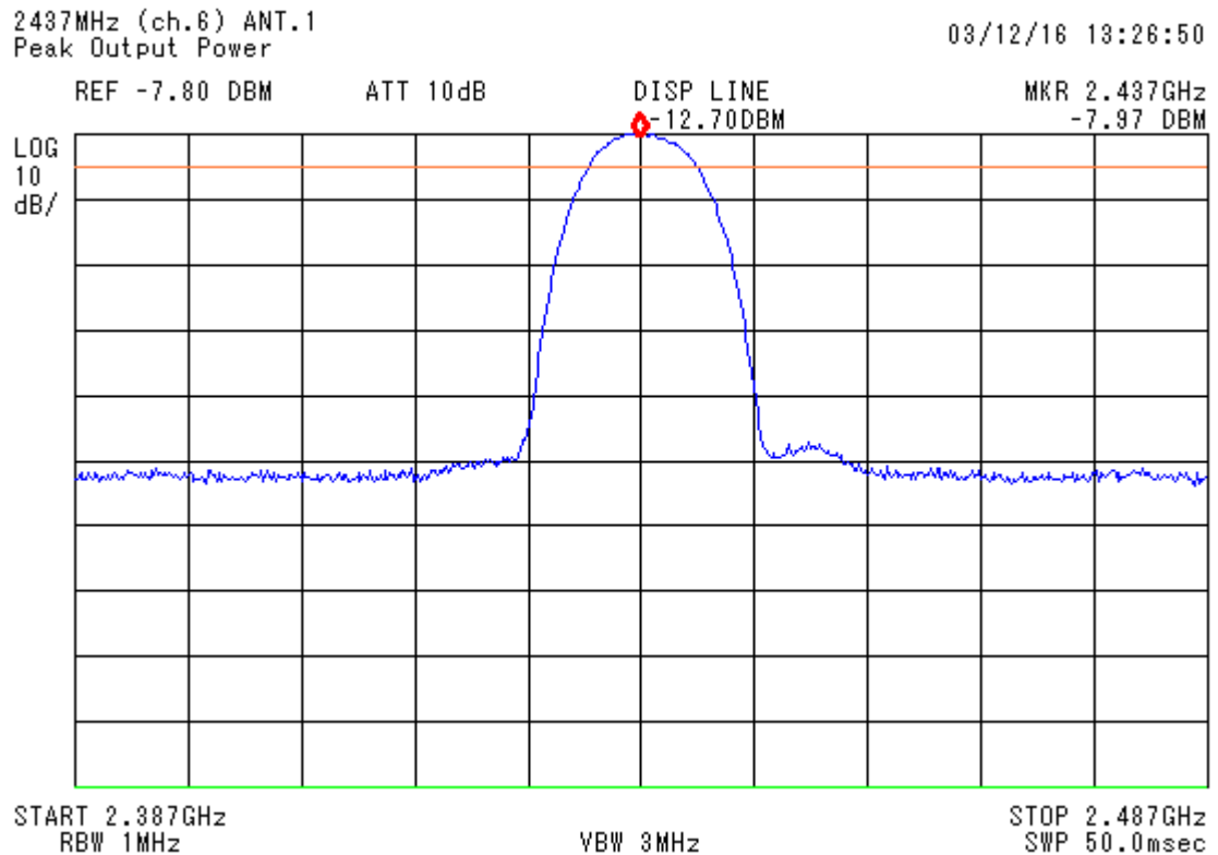
figure 9 2437 MHz_0a (channel 6)
