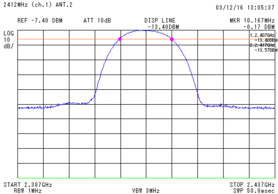
figure 2 6dB Bandwidth fc = 2412 MHz_4a
