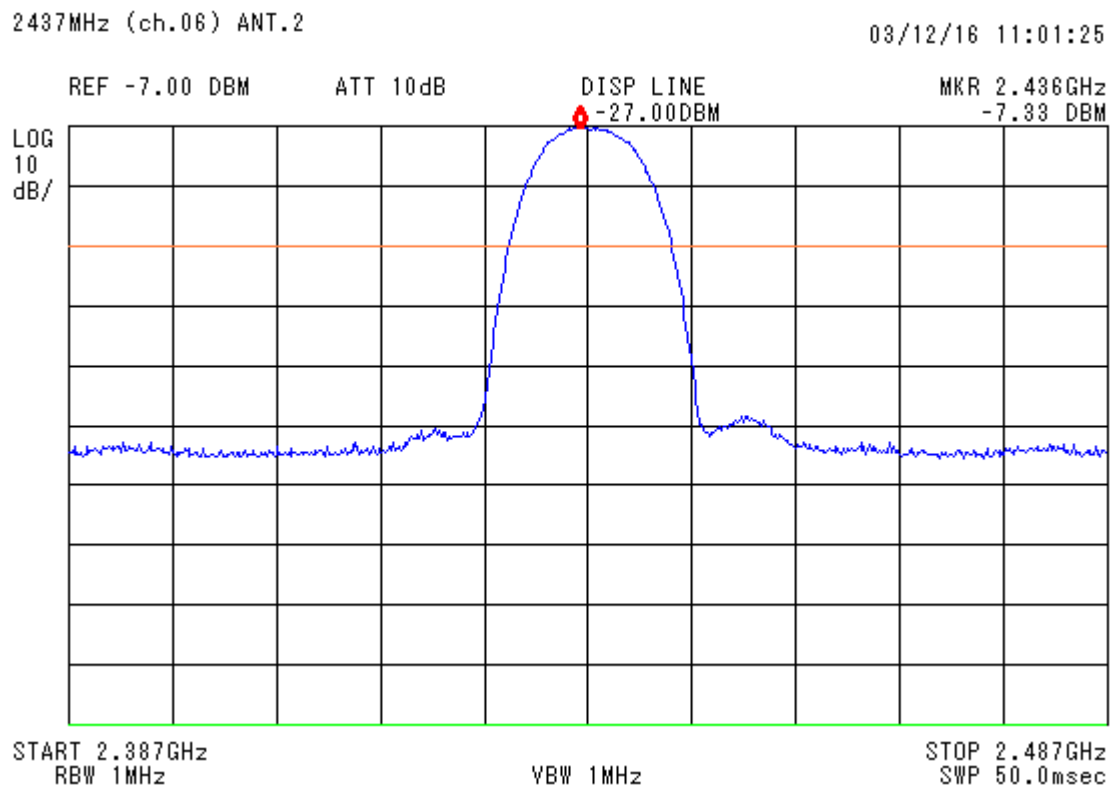
figure 10 2437 MHz_4a (channel 6)
