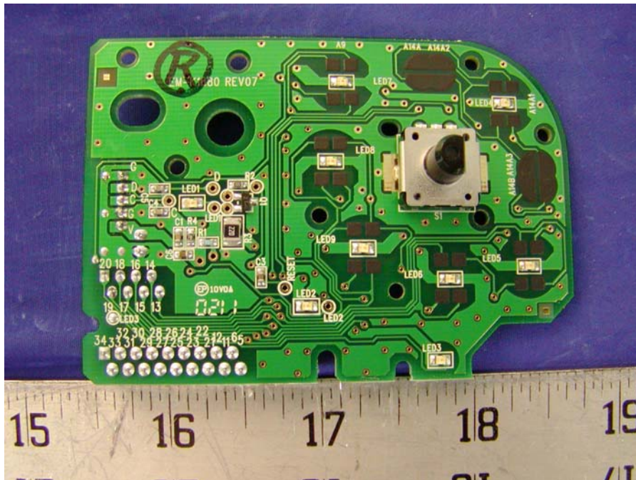
PCB - Component View
