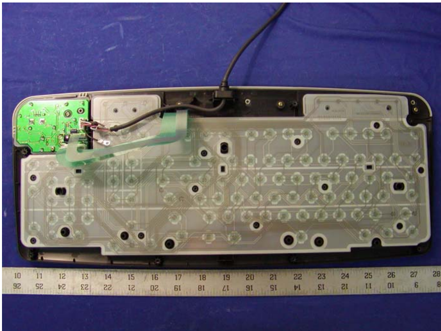
Chassis - Cover Off View 2
