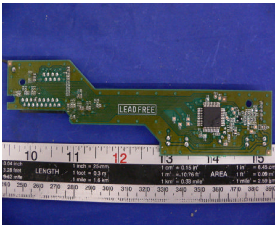
EUT - Component View
