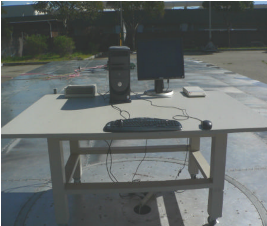
PS2 - Radiated Emission Front View
