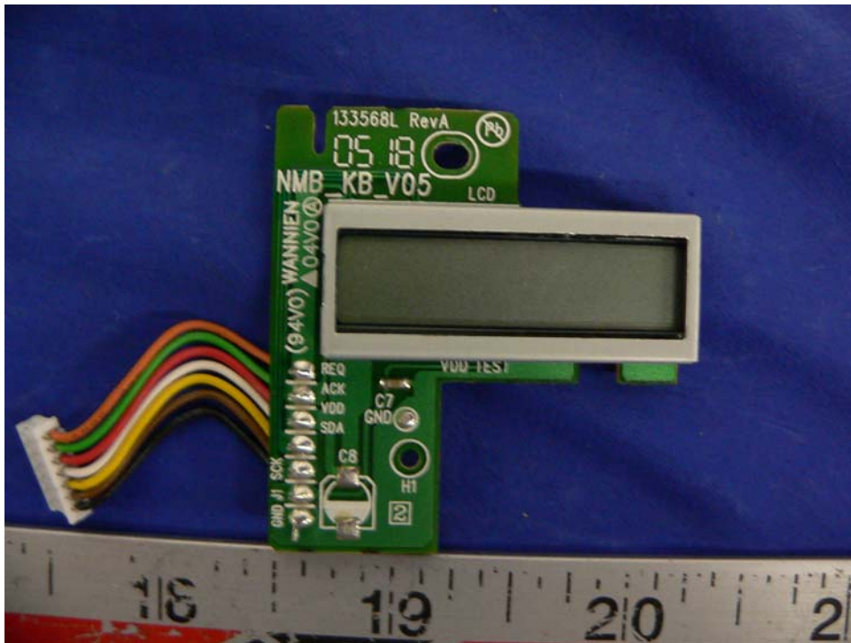
EUT – LCD Board Component View
