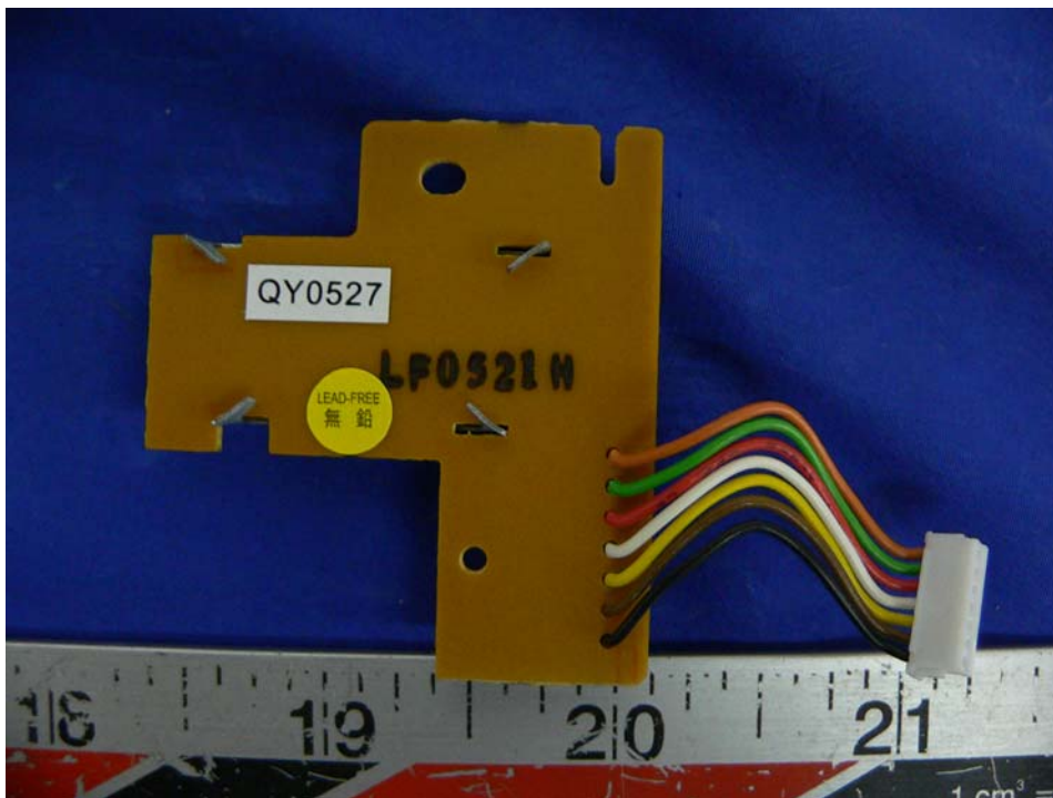
EUT – LCD Board Solder View
