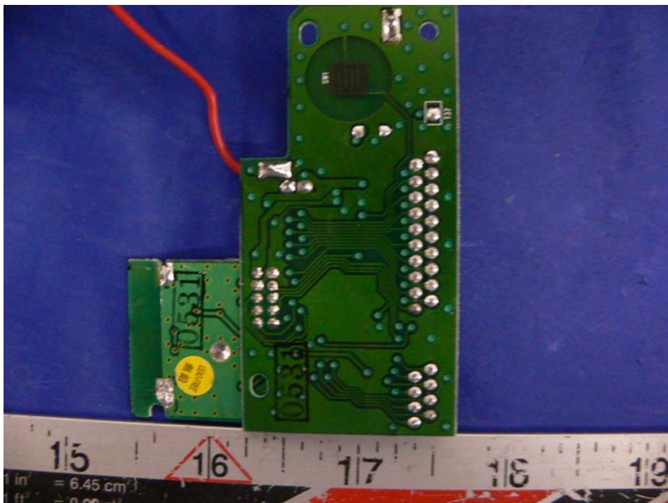
EUT – Board Solder View
