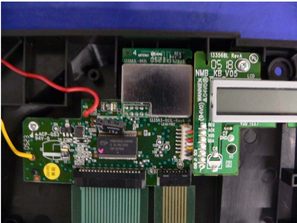
EUT – Main Board View
