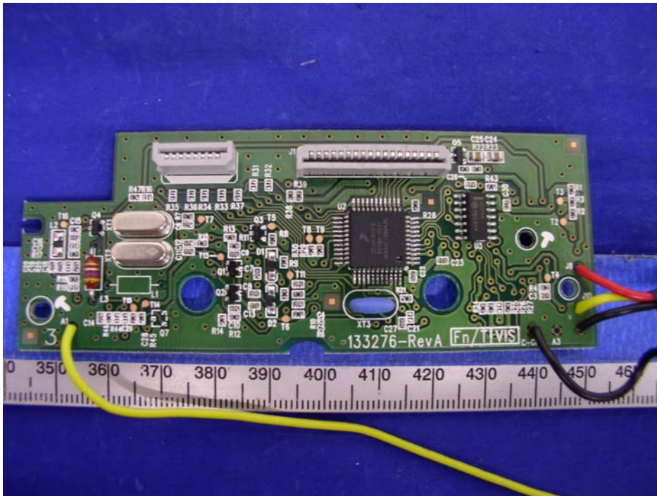
EUT – Component View I
