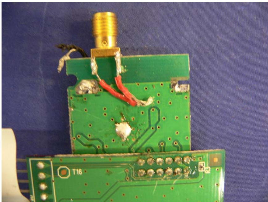
RF Board – Solder View
