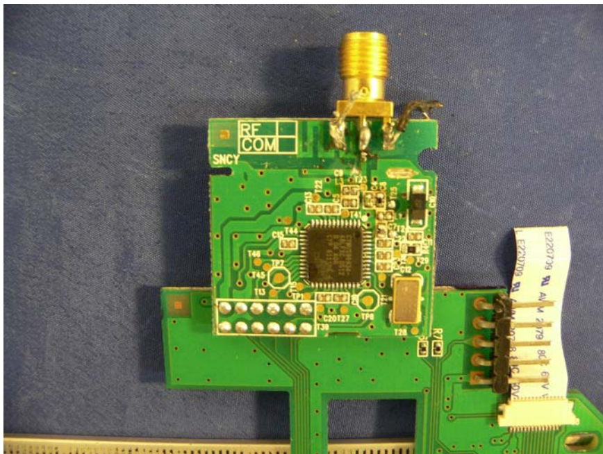
RF Board – Transmitter Cover off, Component and Antenna View
