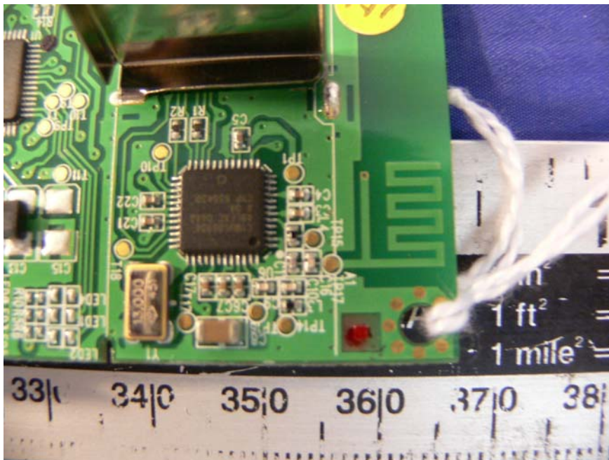
EUT – RF Shielding off View
