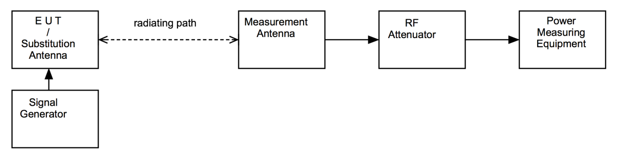
Figure vii Test Setup
