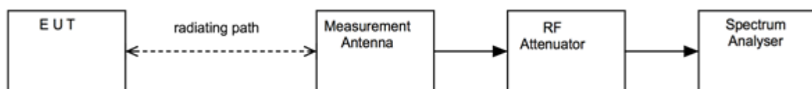
Figure iv Test Setup
