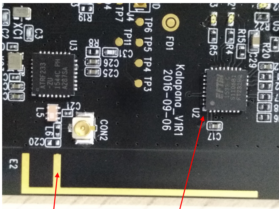
802.15.4 ANTENNA
