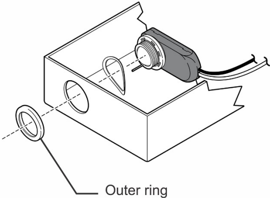
Figure 6: Sensor attachment to fixture
