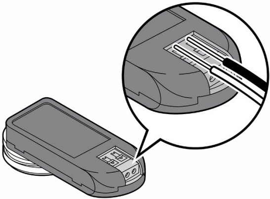
Figure 5: Wire stripping detail
