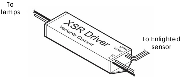
Figure 4: Wiring Connection
