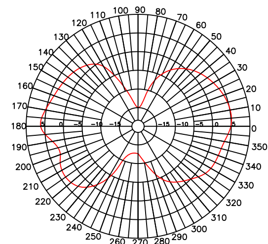
E-Plane Pattern @ 2.45GHz
