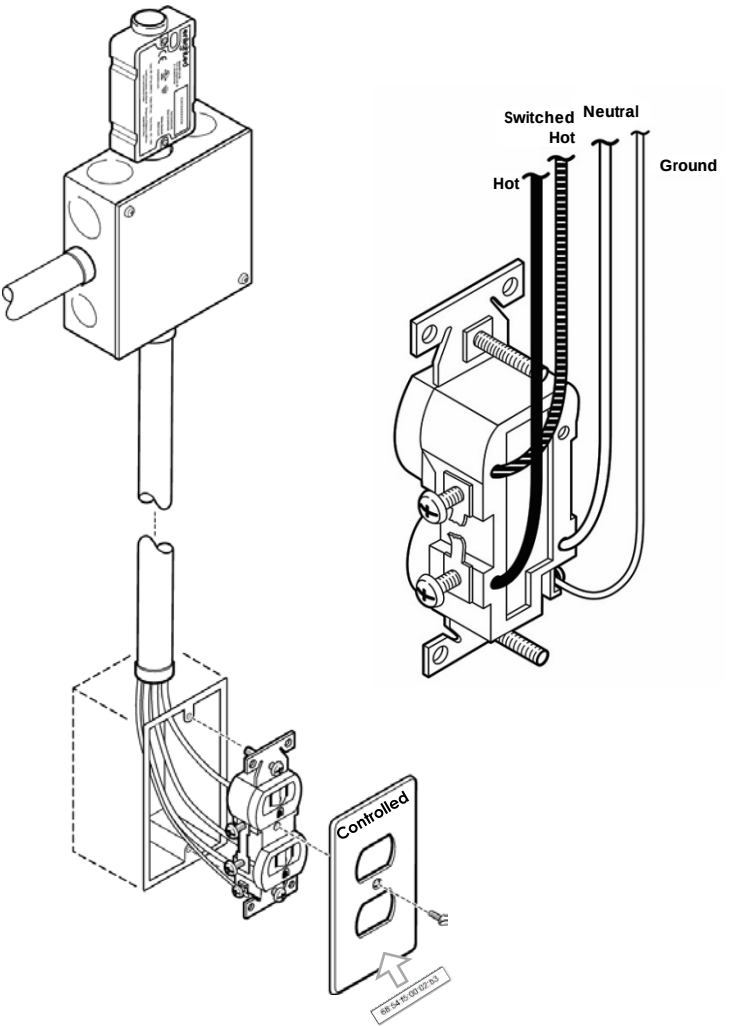
Figure 4: Receptacle wiring
