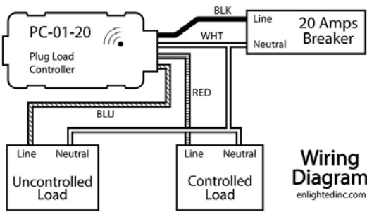
Figure 3: Wiring Diagram
