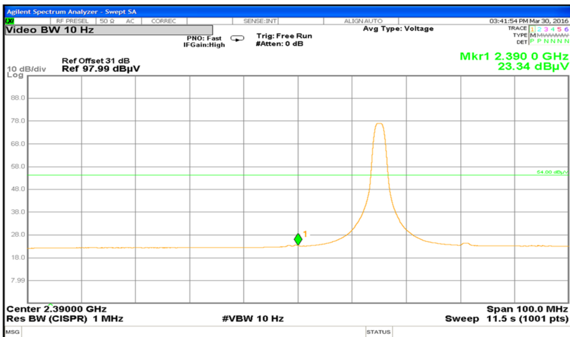
Figure 41: Radiated Emission at the 2390MHz Channel 2405 MHz at – Horizontal (Avg)
