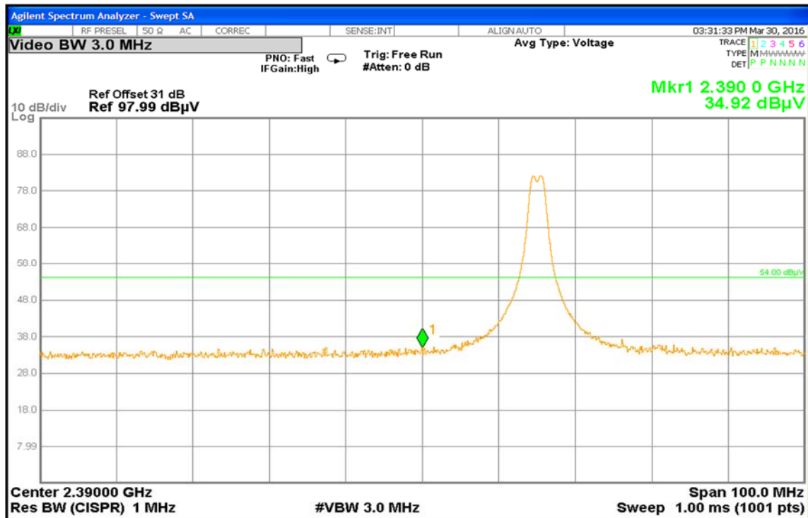
Figure 40: Radiated Emission at the 2390MHz Channel 2405 MHz at – Horizontal (Pk)
