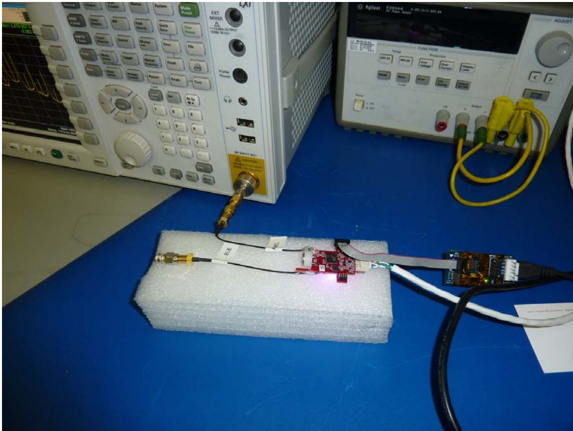
Figure 8: Conducted RF Test Setup (Closer View)
