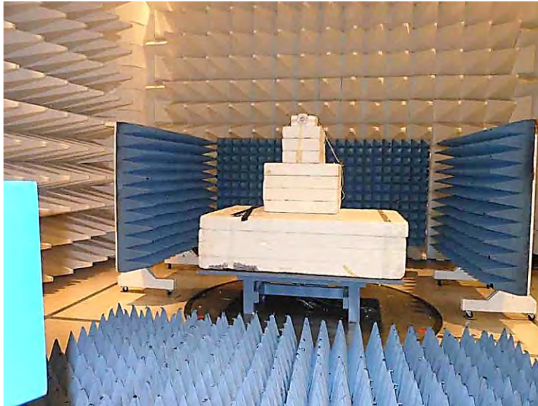
Configuration 1, 12 – 18GHz
