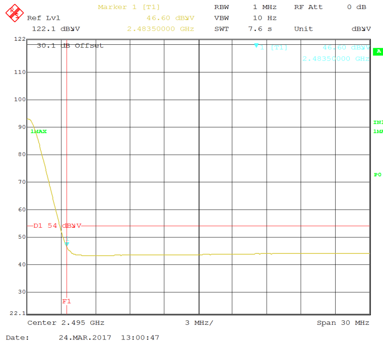
Figure 31: Radiated Emission at 2483.5 MHz Edge – 2480-2510MHz – BLE – Horz. (Ave)
