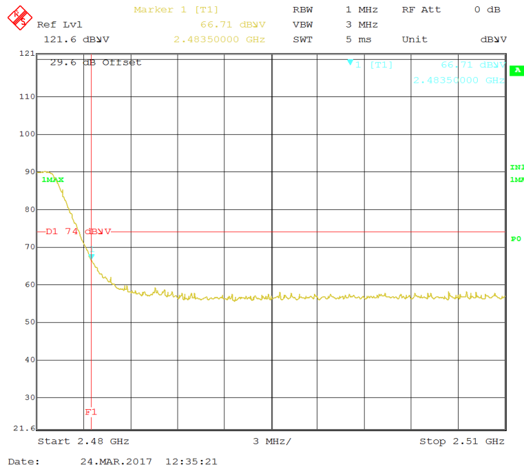
Figure 37: Radiated Emission at 2483.5 MHz Edge – 2480-2510MHz – IEEE 802.15.4 – (Peak)
