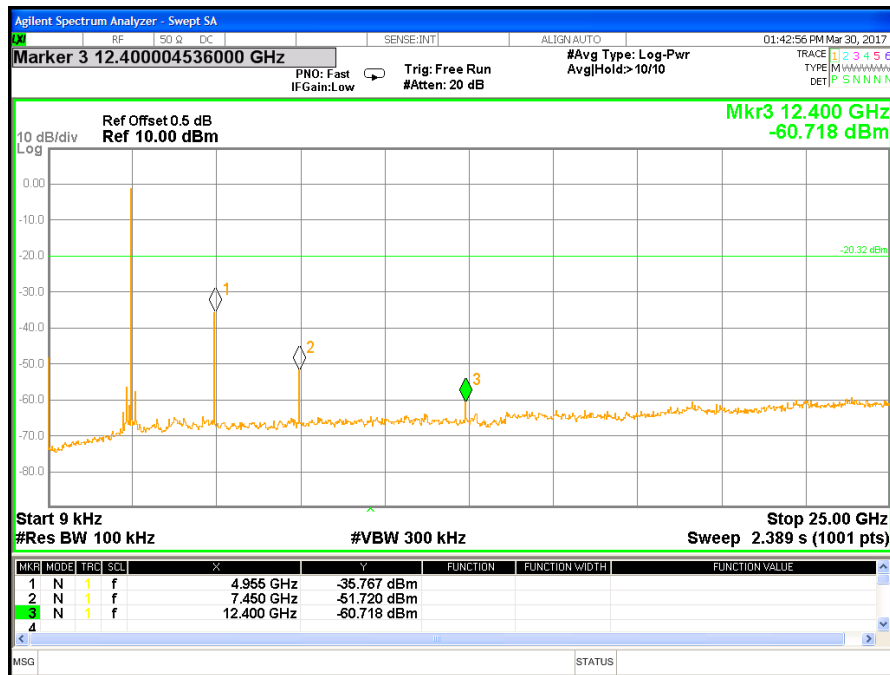
Figure 23: Out of Band Emissions at 2480 MHz, 9kHz-25GHz – BLE
