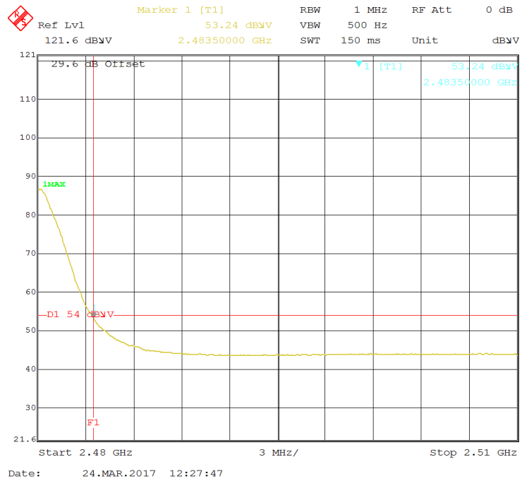
Figure 35: Radiated Emission at 2483.5 MHz Edge – 2480-2510MHz – Zigbee – Horz. (Ave)
