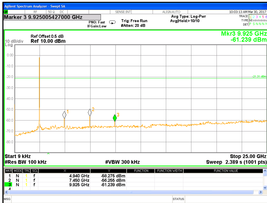
Figure 28: Out of Band Emissions at 2480 MHz, 9kHz-25GHz – IEEE 802.15.4
