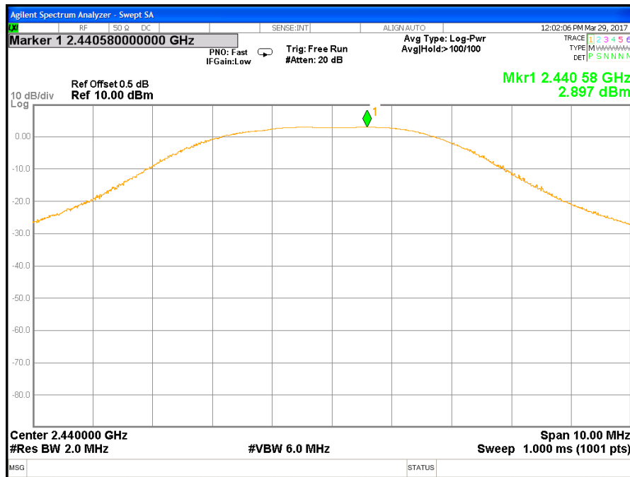
Figure 5 : Maximum peak conducted output power – IEEE 802.15.4 – 2440MHz
