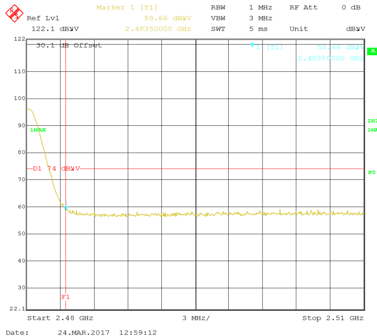
Figure 32: Radiated Emission at 2483.5 MHz Edge – 2480-2510MHz – BLE – Horz. (Peak)
