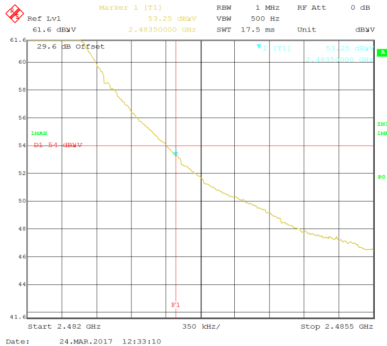
Figure 36: Radiated Emission at 2483.5 MHz Edge – 2482-2485.5MHz – IEEE 802.15.4 – (Peak)
