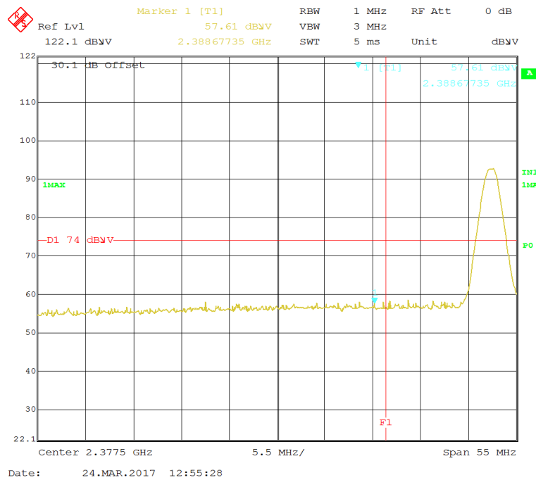
Figure 30: Radiated Emission at 2390 MHz Edge – 2350-2405MHz – BLE – Horz. (Peak)
