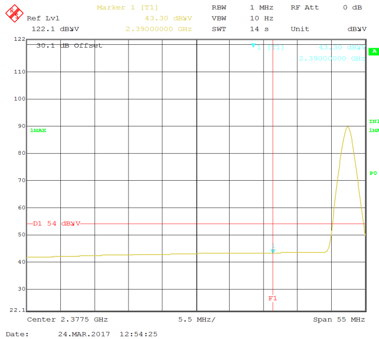
Figure 29: Radiated Emission at 2390 MHz Edge – 2350-2405MHz – BLE – Horz. (Ave)
